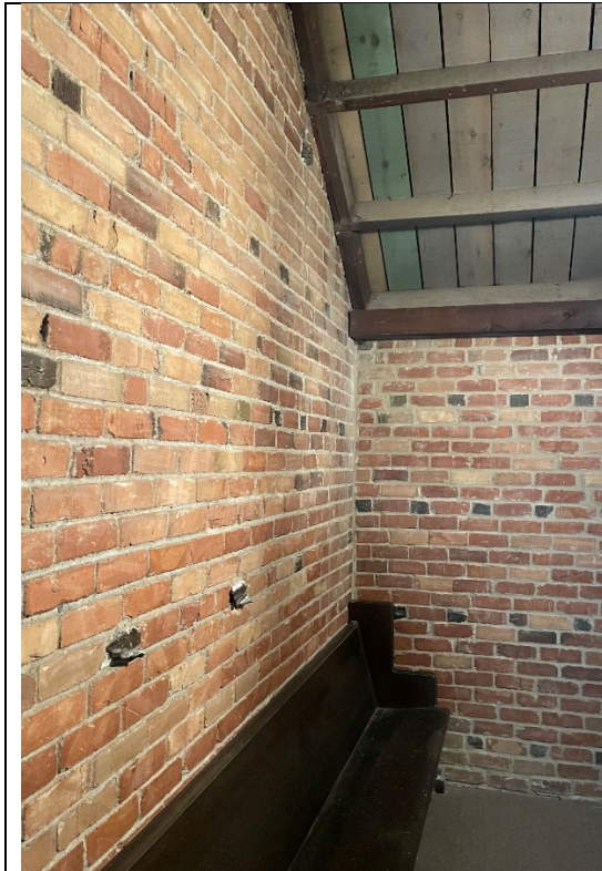
Structural brick repair and re-pointing: Brick walls had structural cracking in multiple locations and were restored in the preservation project.
