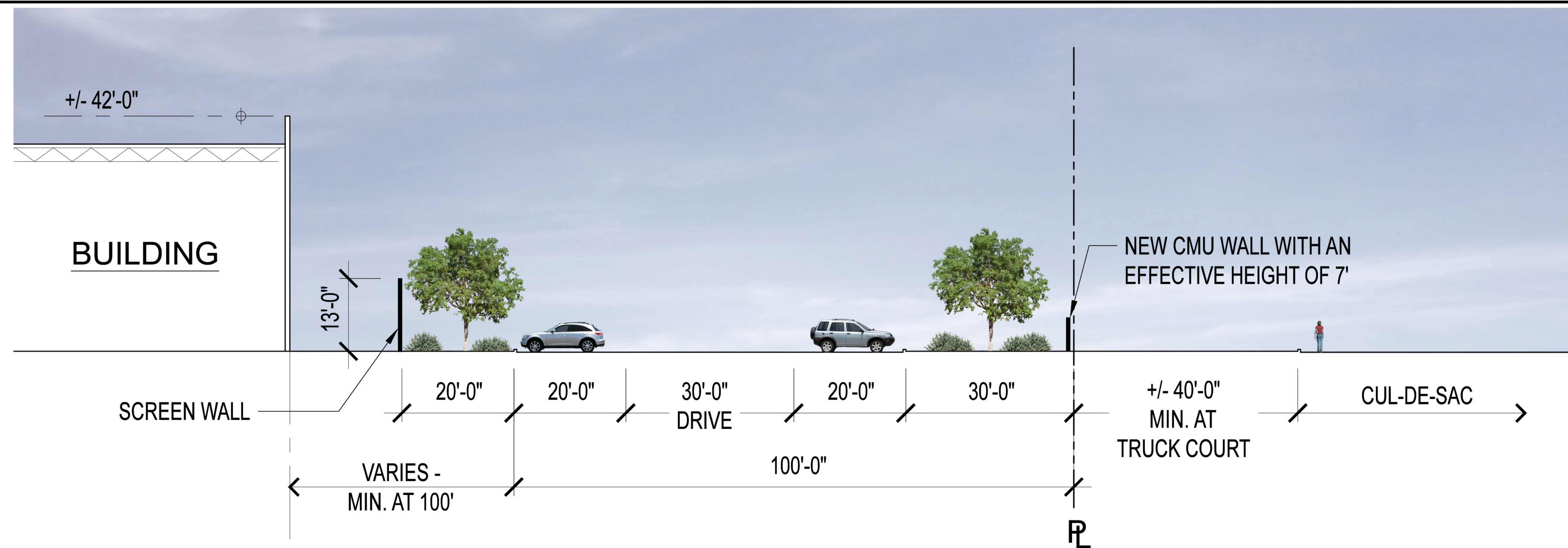
PRELIMINARY SITE SECTION - 1
