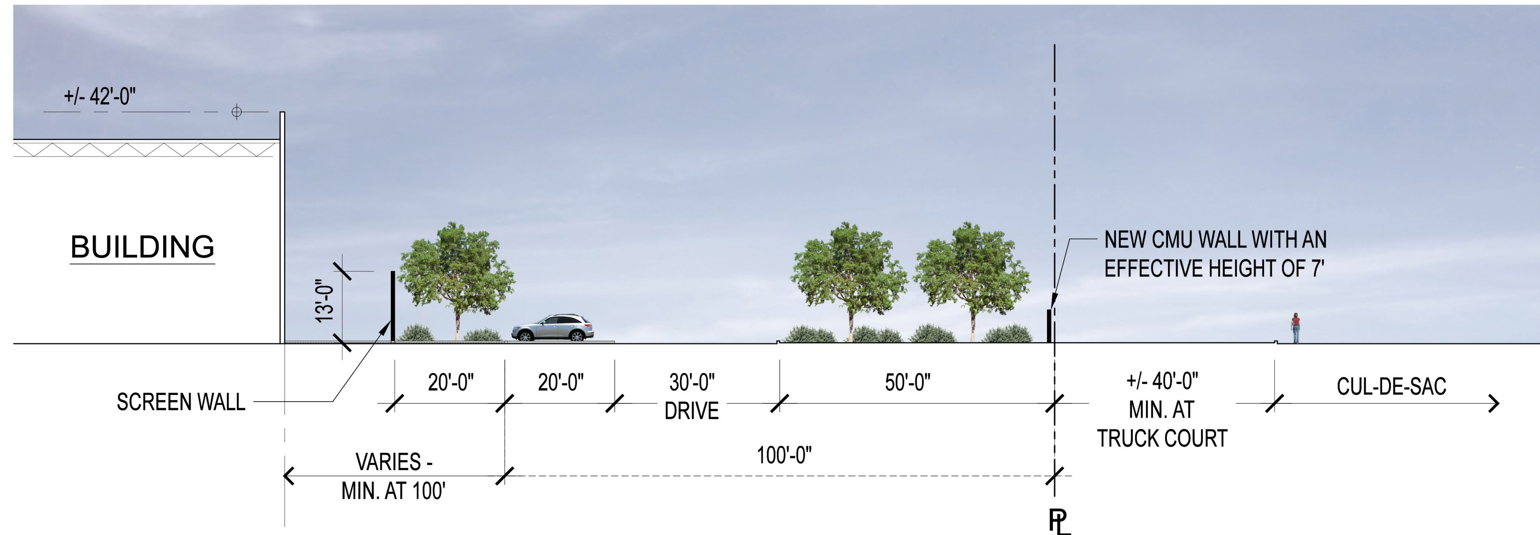
PRELIMINARY SITE SECTION - 2
