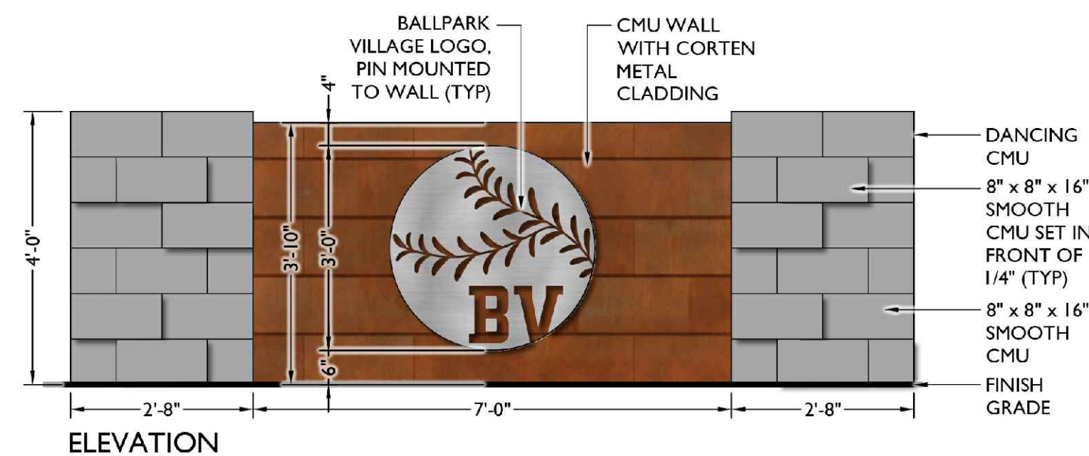
2 SECONDARY REGIONAL MONUMENT Scale: 1/2" = 1'-0"
