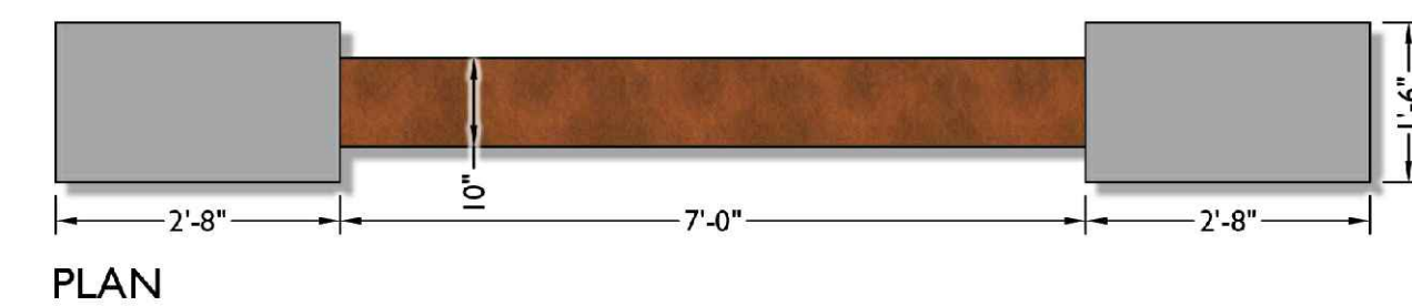
1 PRIMARY REGIONAL MONUMENT Scale: 1/2" = 1'-0"
