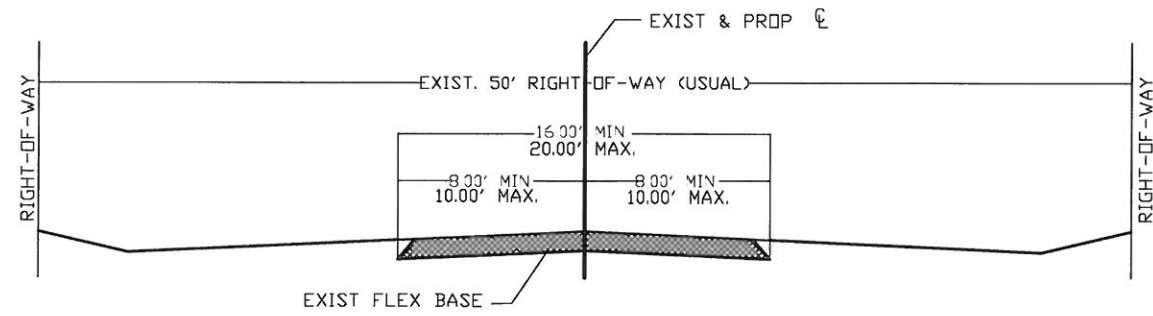
EXISTING TYPICAL STREET SECTION
