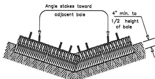
PROFILE VIEW
