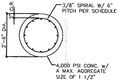
SECTION X-X
