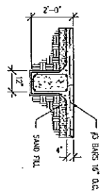
B-INTERIOR BEAM
