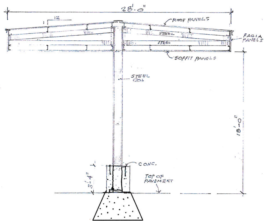
CANOPY SECTION 4"=1'-0"
