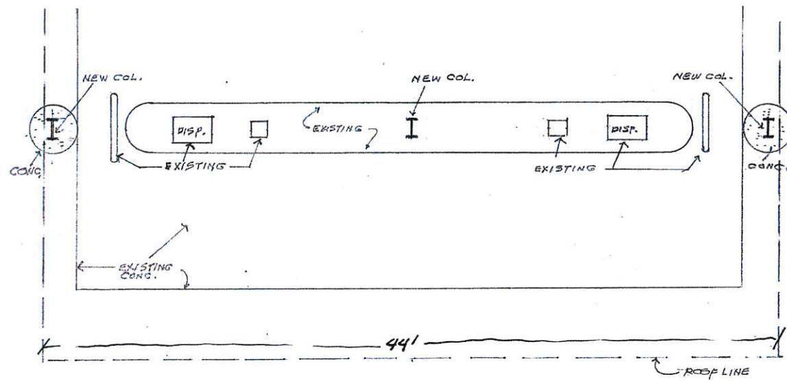
CANOPY PLAN 1/4"=1'-0"
