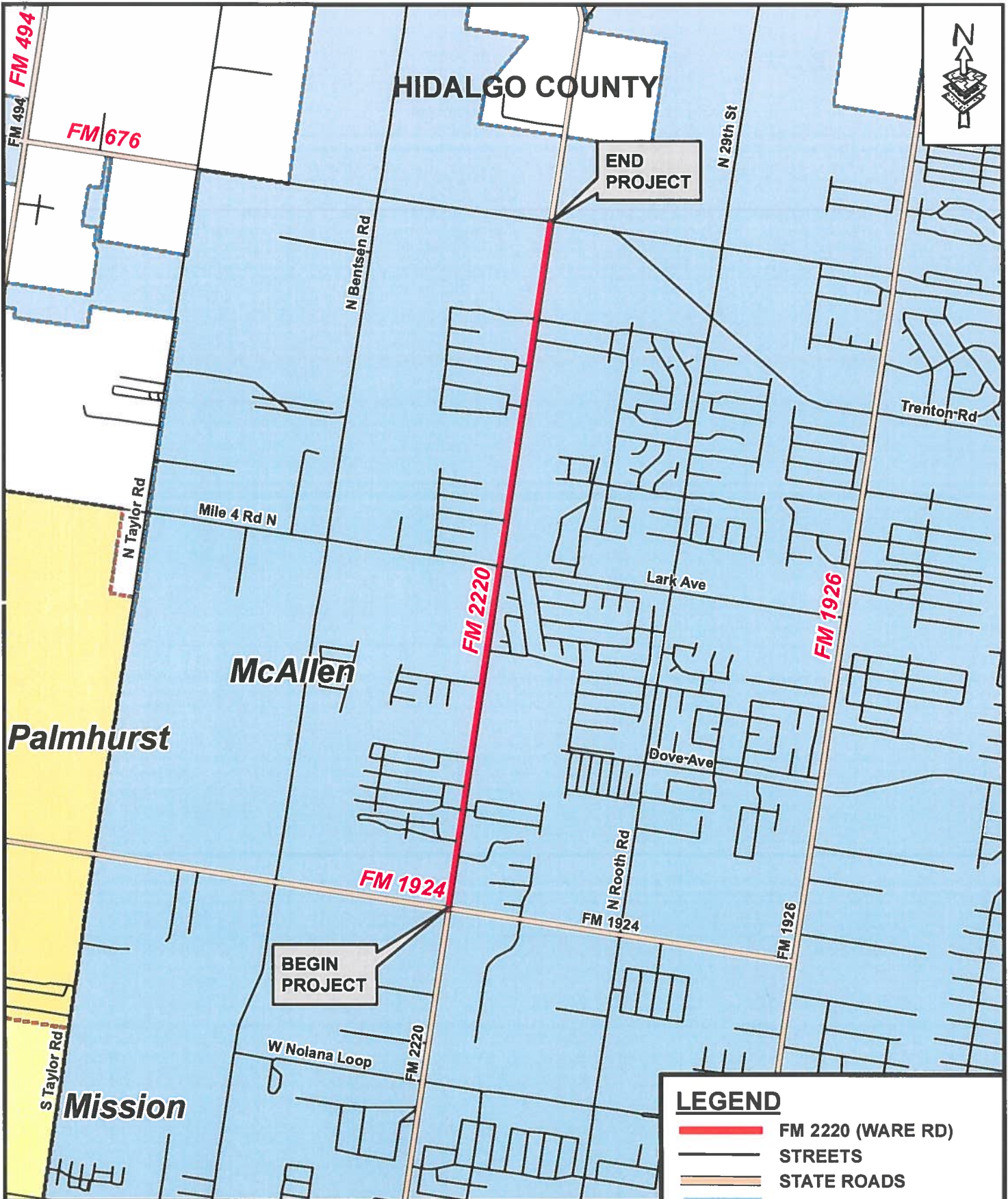
FM 2220 (WARE RD) LOCATION MAP FROM FM 1924 (MILE 3) TO MILE 5 NORTH APPROX. PROJECT LENGTH 2.0 MILES
