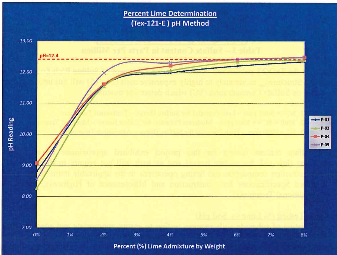
Figure 5 – Lime Series Testing Graph
