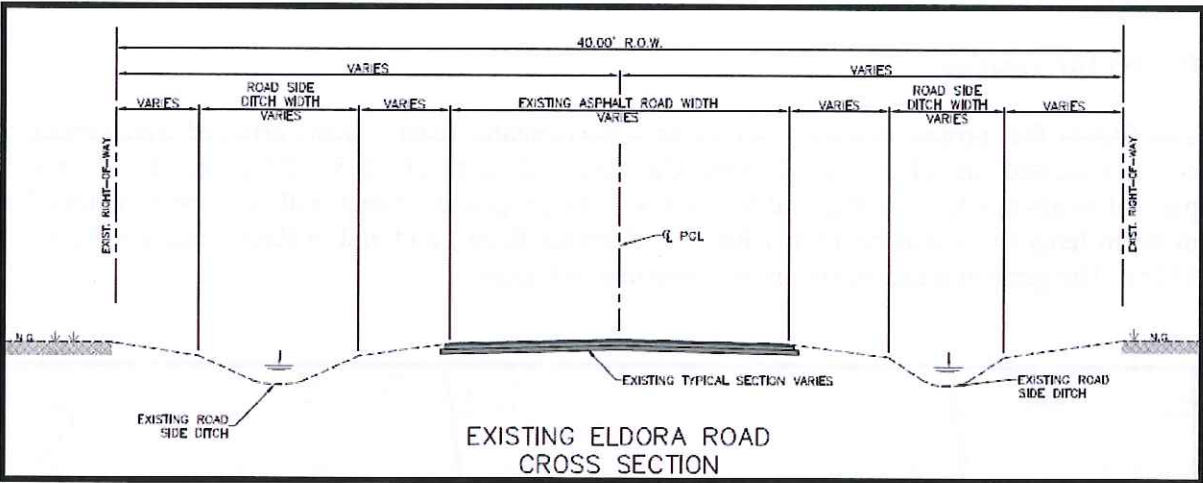
Figure 2A – Eldora Rd. Project Existing Typical Section
