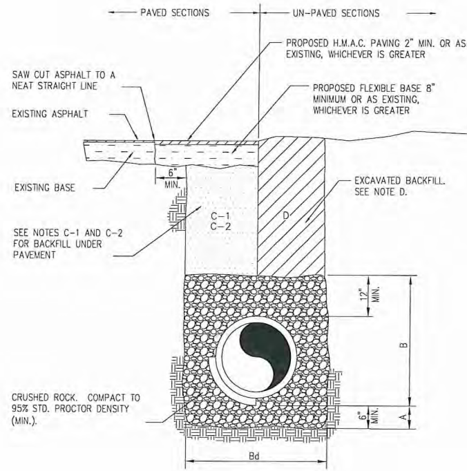
SANITARY SEWER (NON-FORCEMAIN) PIPE BEDDING DETAIL N.T.S.
