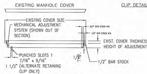
MANHOLE COVER ADJUSTMENT DETAILS N.T.S.
