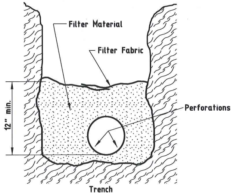
Figure 1 Installation Process
