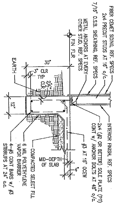
A-EXTERIOR BEAM
