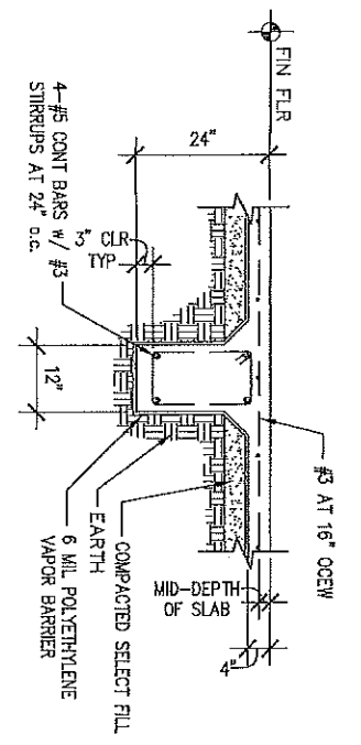
B-INTERIOR BEAM
