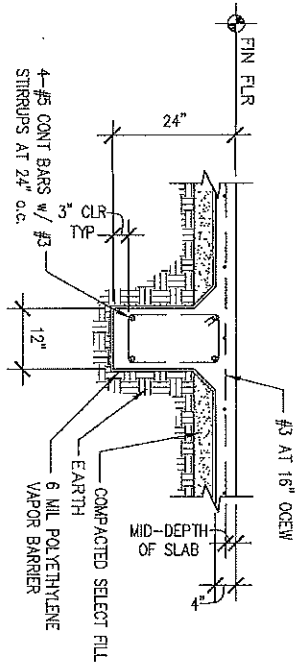
B-INTERIOR BEAM
