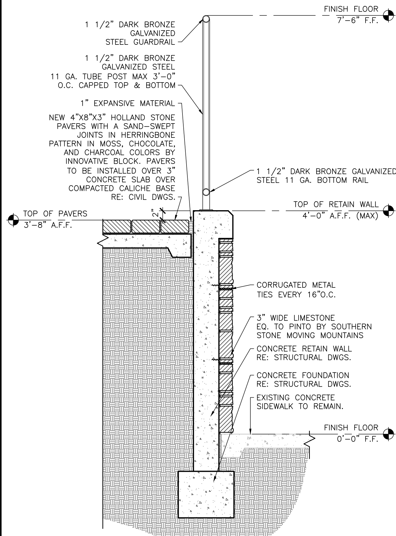
6 RETAINING WALL SECTION DETAIL
