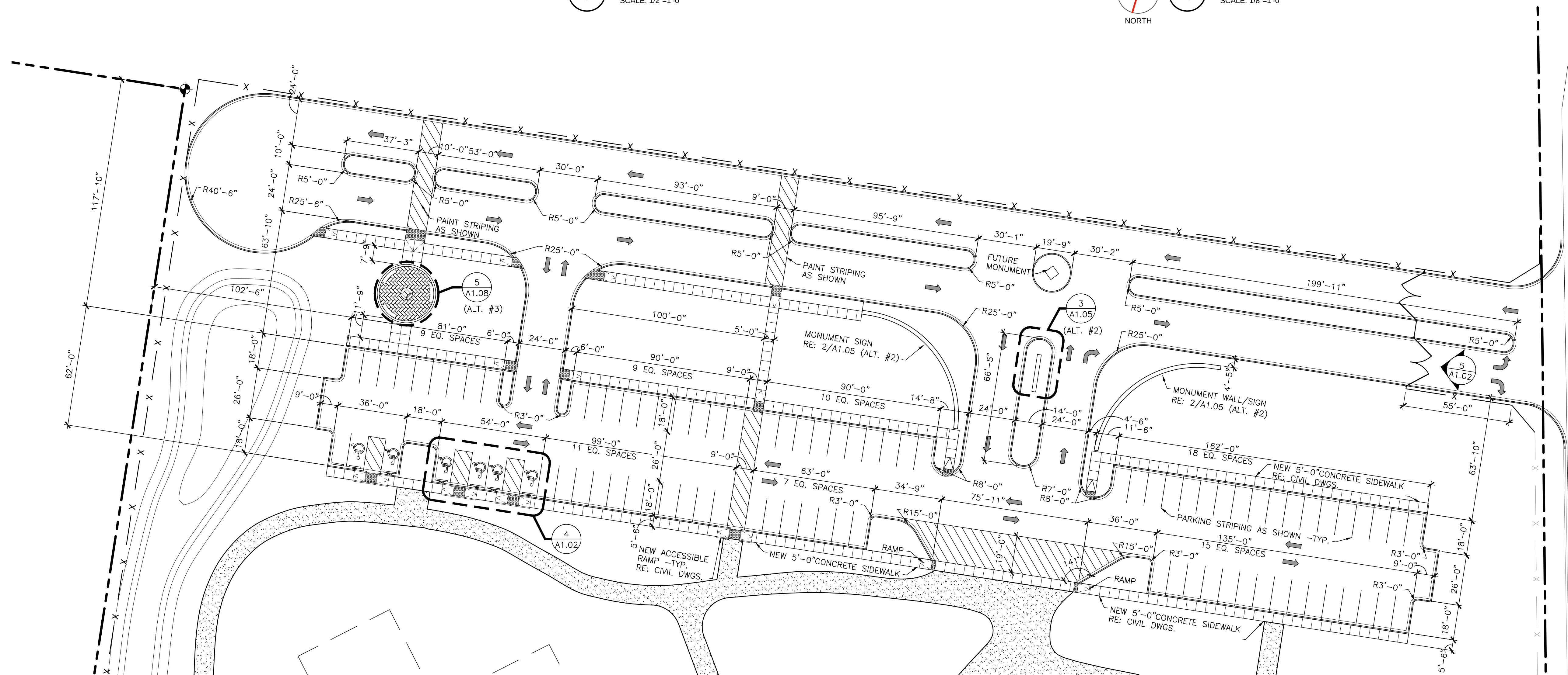
ALT. 1 - PARTIAL SITE AT NEW PARKING LOT
