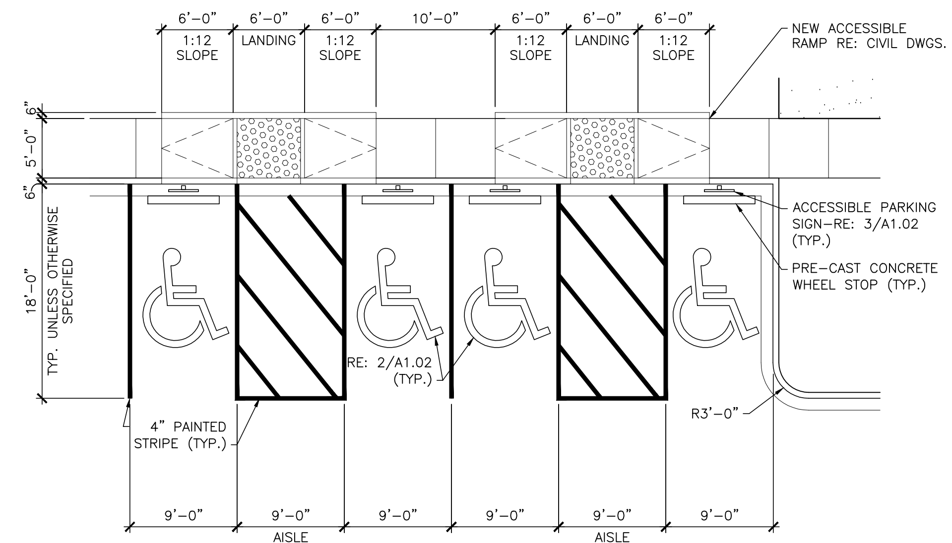
4 ACCESSIBLE PARKING DETAIL
