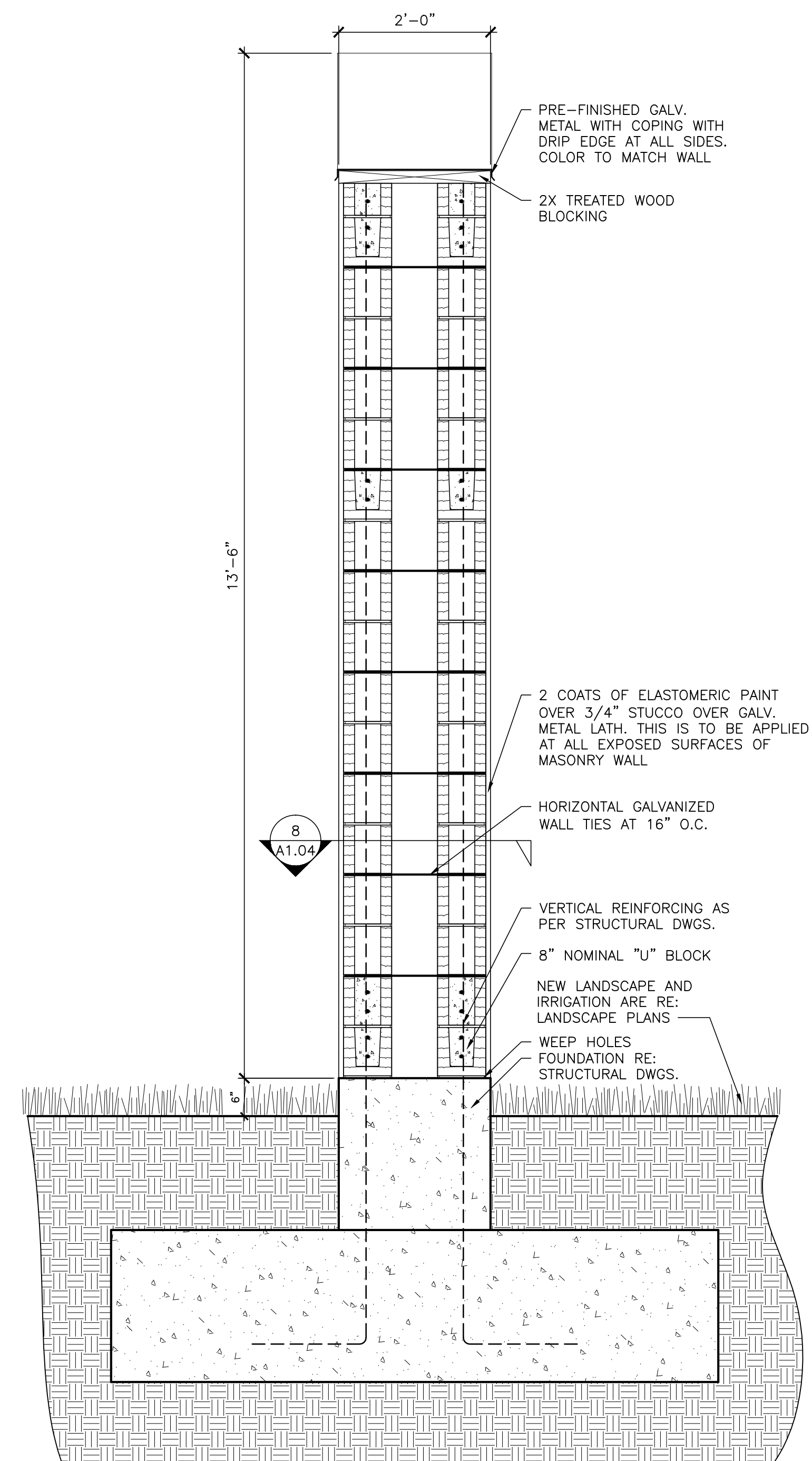
7 MONUMENT SIGN SECTION DETAIL SCALE: 3/4"=1'-0"
