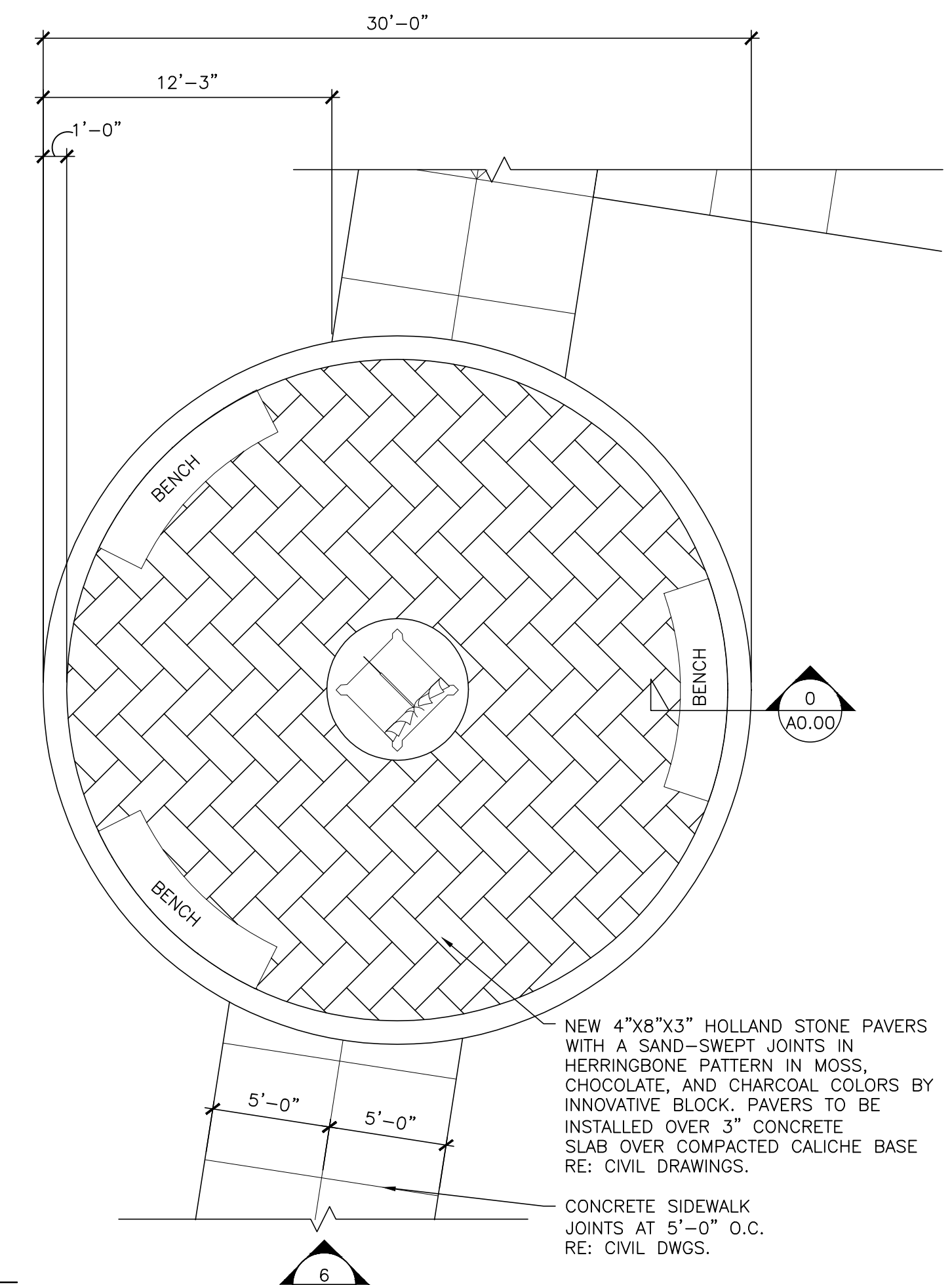
5 ALT. 3 - PARTIAL SITE PLAN AT WINDMILL MEMORIAL SCALE: 3/16"=1'-0"
