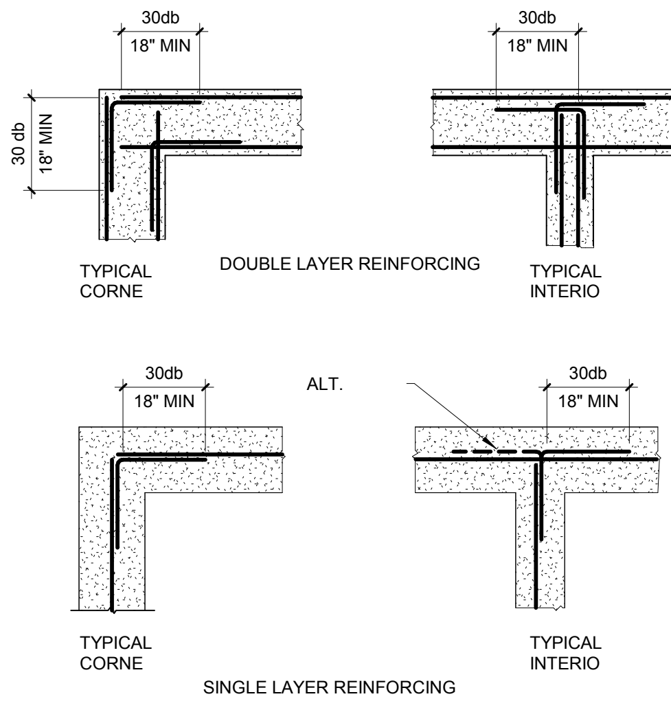
Typical Reinforcing at Concrete Intersections
