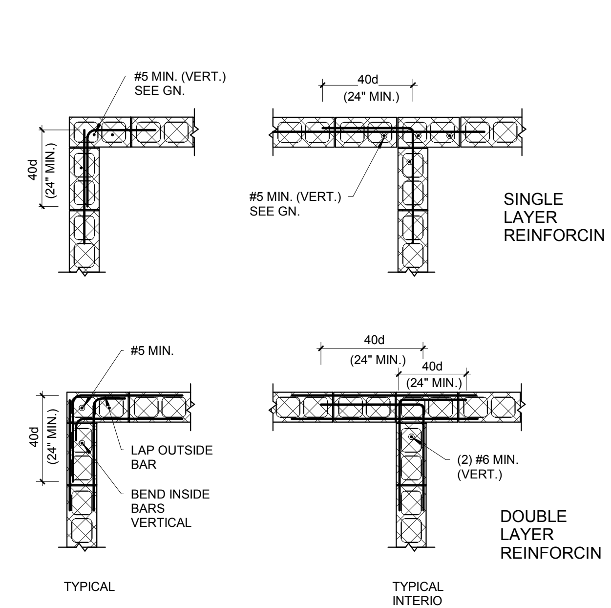
Typical CMU Reinforcing at Intersections 1/2" = 1'-0"
