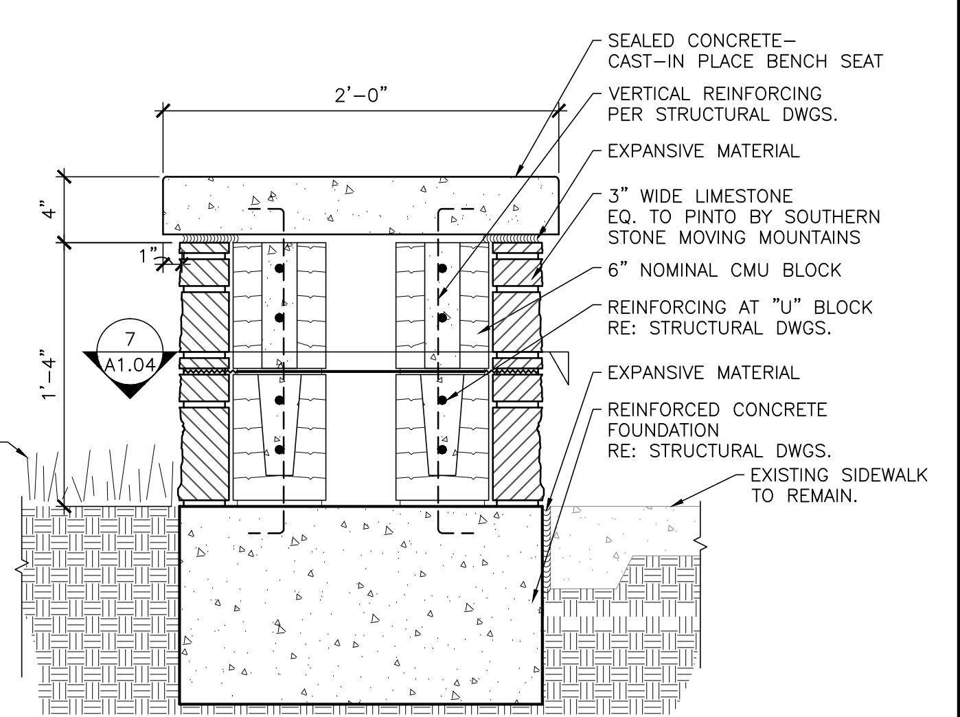
5 TREE WELL BENCH SECTION DETAIL SCALE: 1 1/2"=1'-0"
