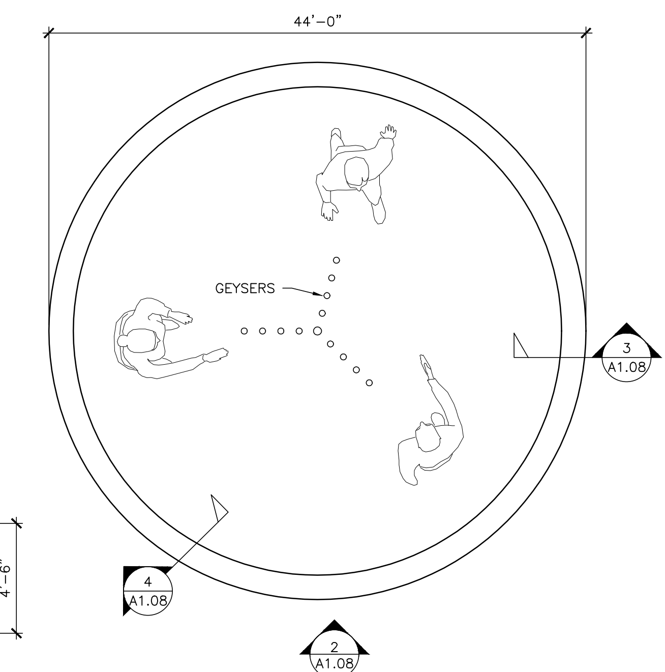
1 ALT. 5 - PARTIAL SITE PLAN AT FOUNTAIN FEATURE SCALE: 1/8"=1'-0"
