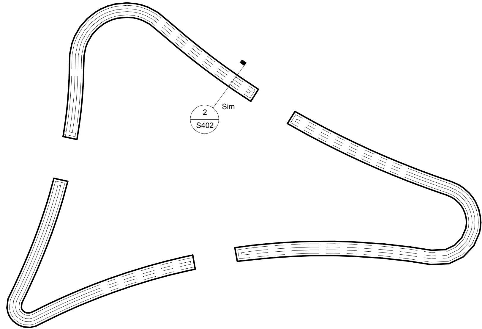
Foundation Plan - Dependent 4 1/8" = 1'-0" S402/S201
