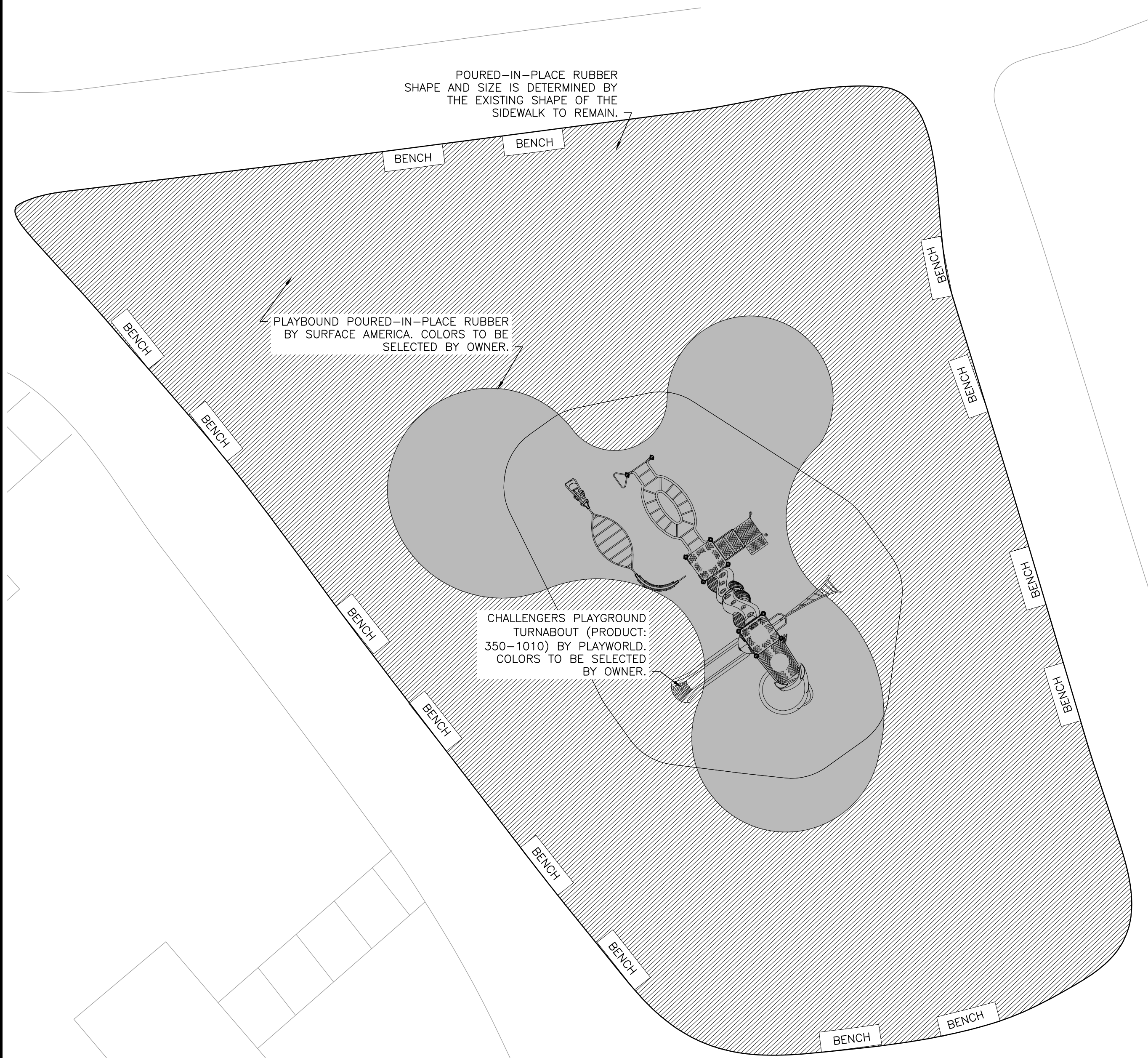
7 PARTIAL SITE PLAN AT PLAYGROUND SCALE: 1/8"=1'-0"
