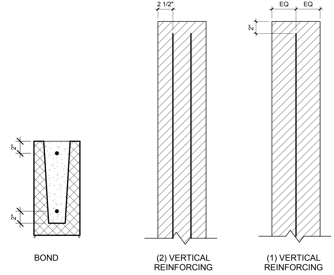
Typical CMU Reinforcing Clearances 1 1/2" = 1'-0"
