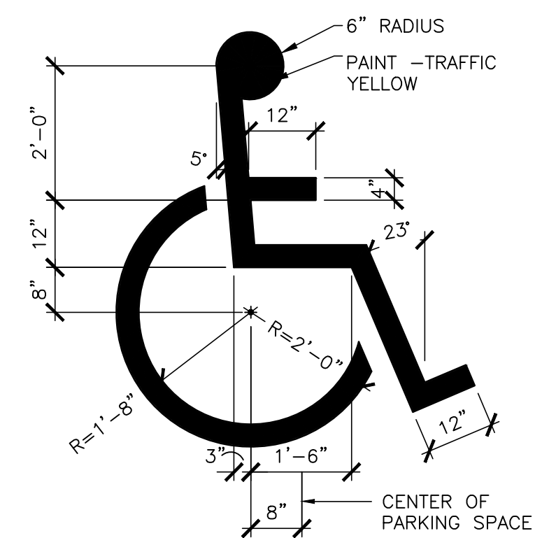
3 ACCESSIBLE SIGN DETAIL
