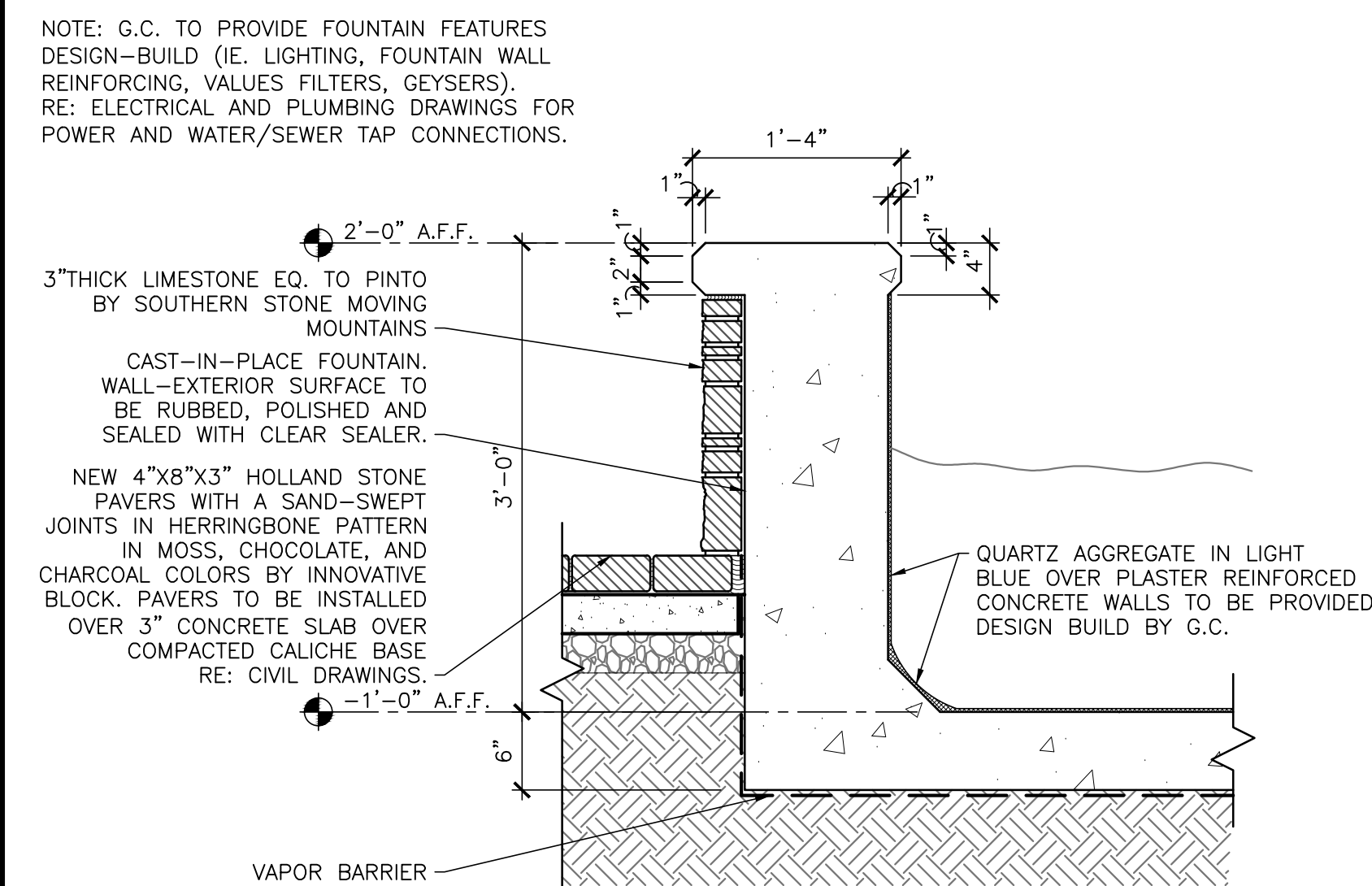
4 FOUNTAIN SECTION DETAIL SCALE: 1/2"=1'-0"
