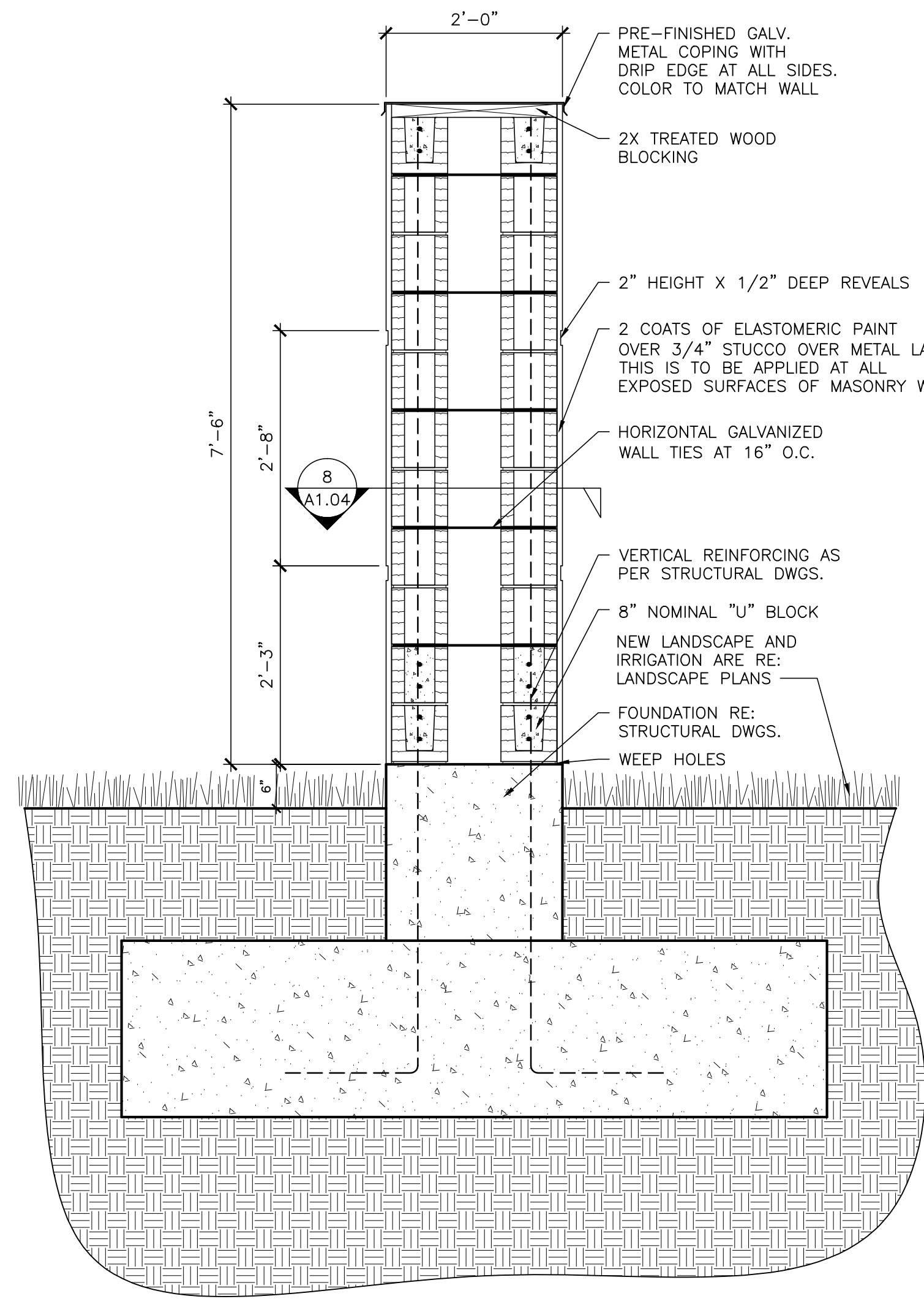
8 MONUMENT SIGN SECTION DETAIL SCALE: 3/4"=1'-0"
