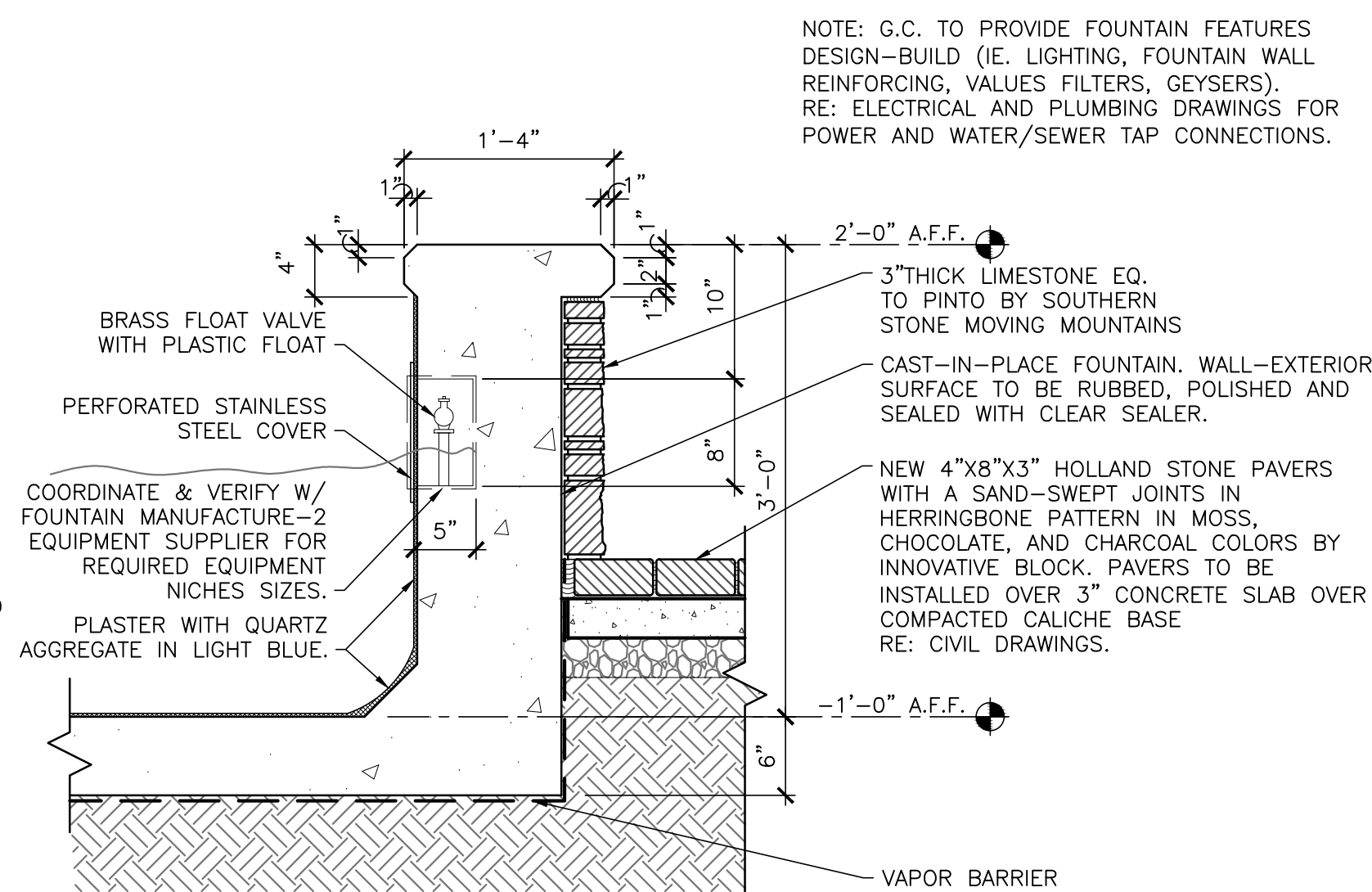
3 FOUNTAIN SECTION DETAIL SCALE: 1/2"=1'-0"
