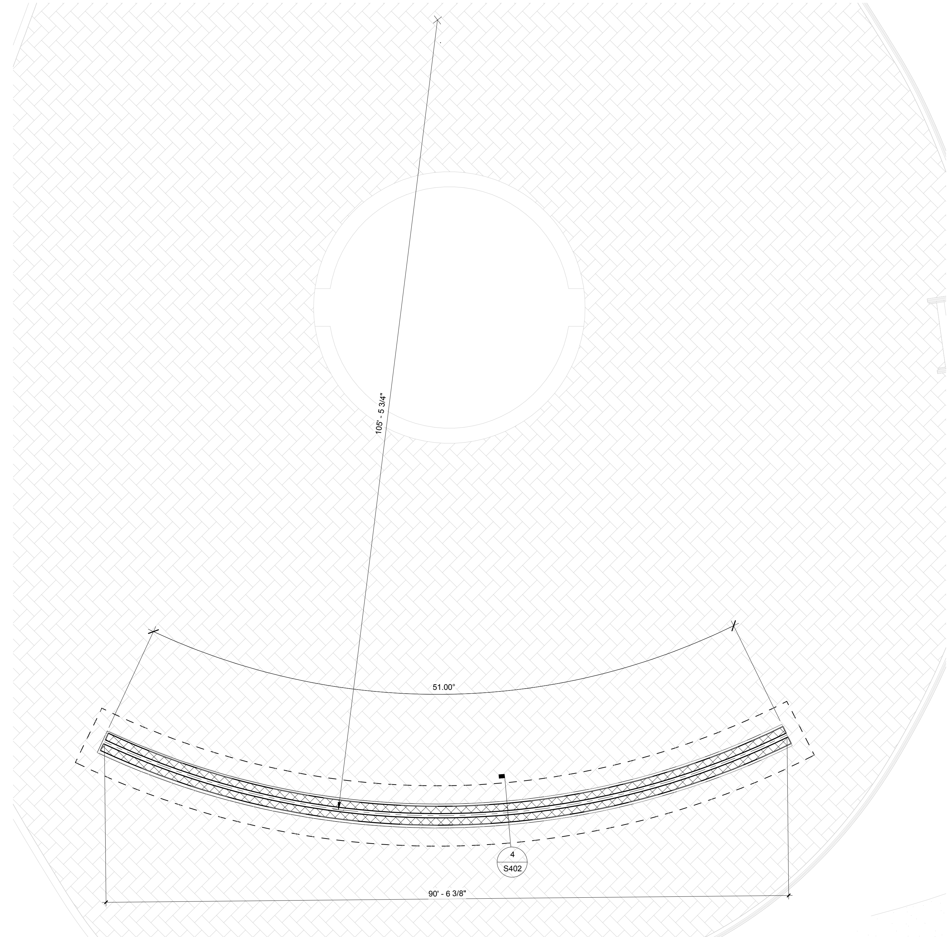
Foundation Plan - Dependent 1 1/8" = 1'-0" S402/S201
