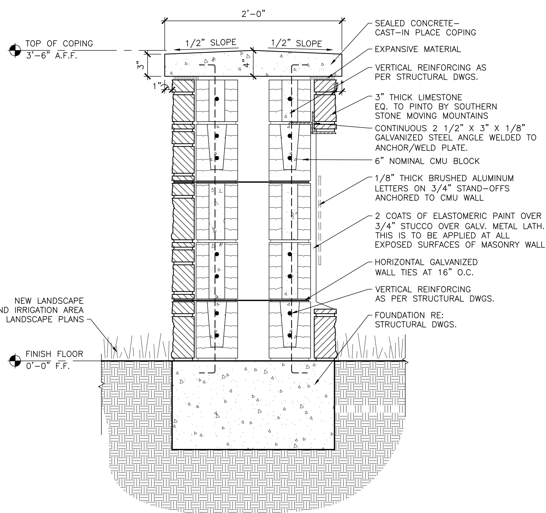
10 MONUMENT WALL SECTION DETAIL SCALE: 1 1/2"=1'-0"
