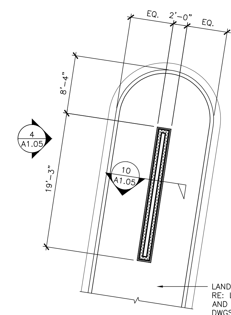
3 ALT. 2- PARTIAL SITE PLAN AT MONUMENT SCALE: 1/8"=1'-0"
