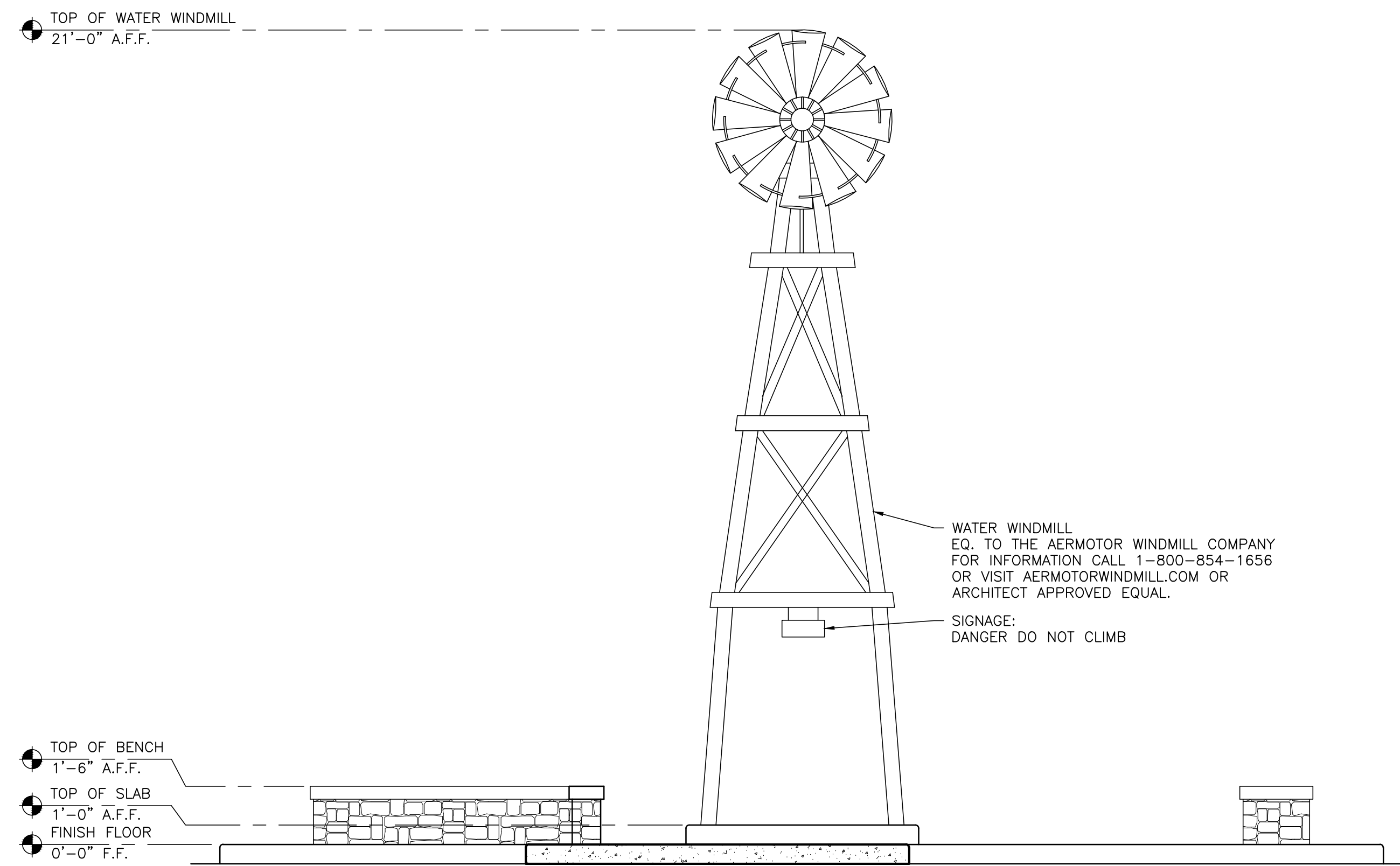
6 ALT. 3 - WINDMILL MEMORIAL ELEVATION SCALE: 3/8"=1'-0"
