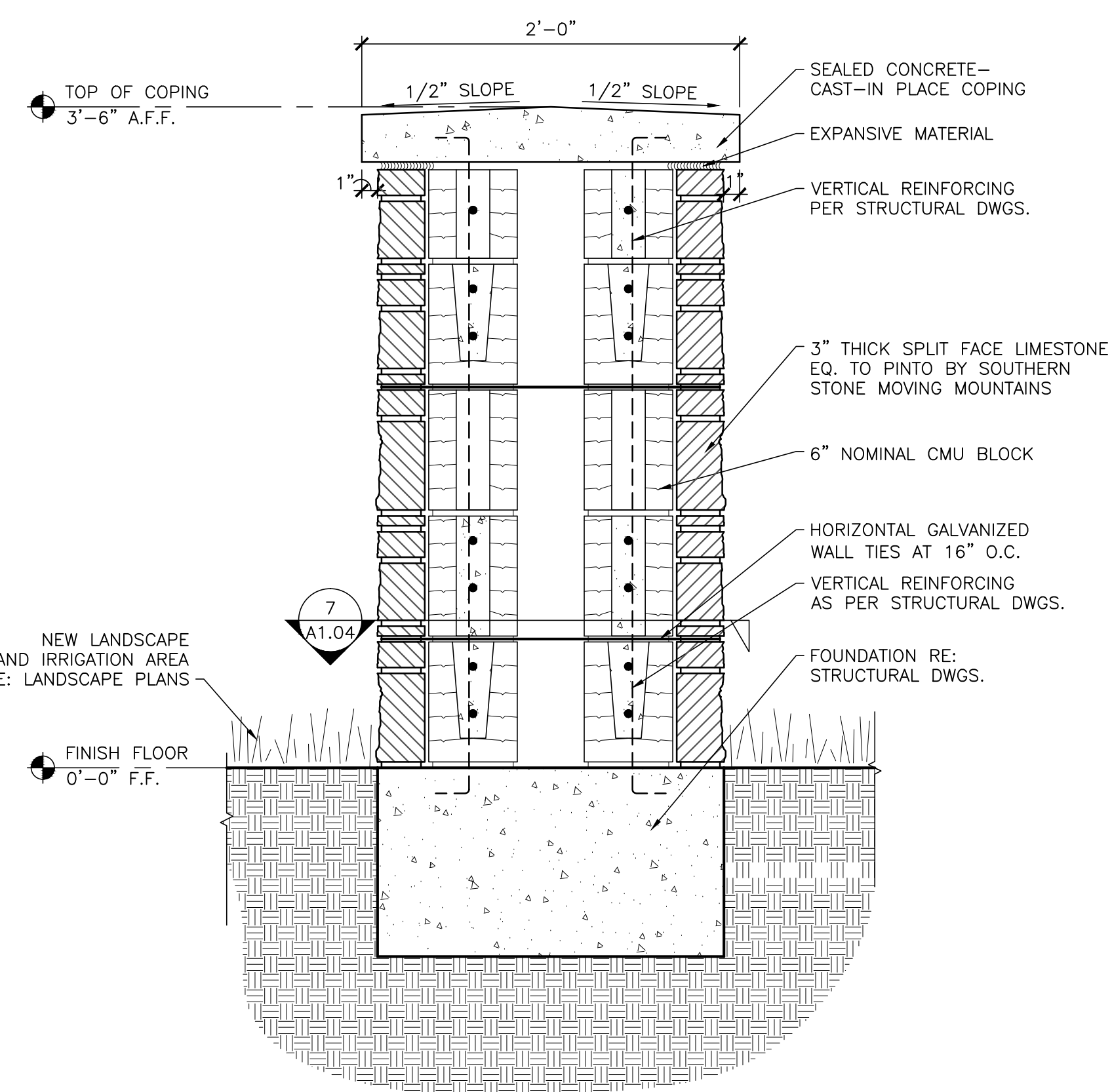
9 MONUMENT WALL SECTION DETAIL SCALE: 1 1/2"=1'-0"
