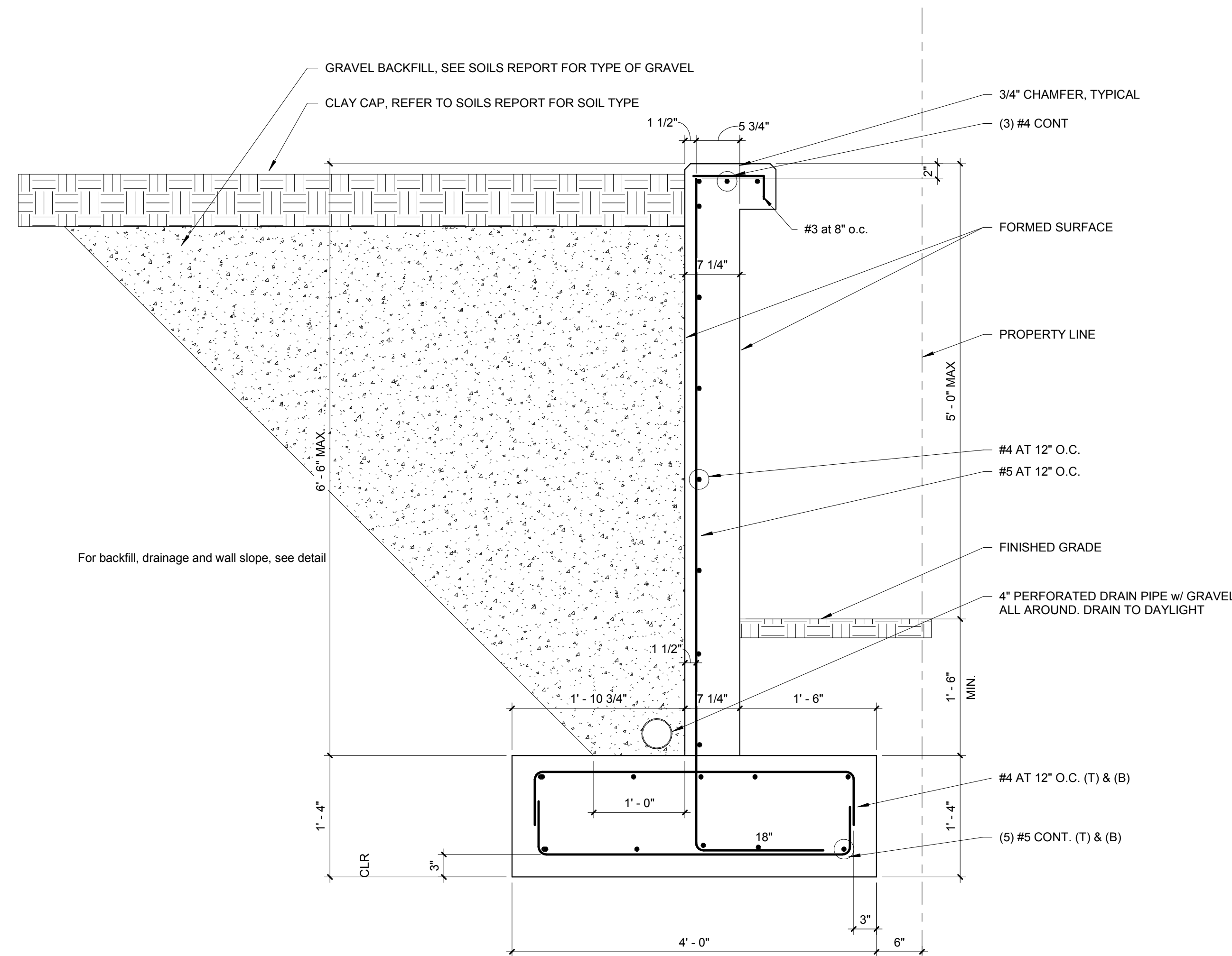
5' Retaining Wall, NO Surcharge 1" = 1'-0"
