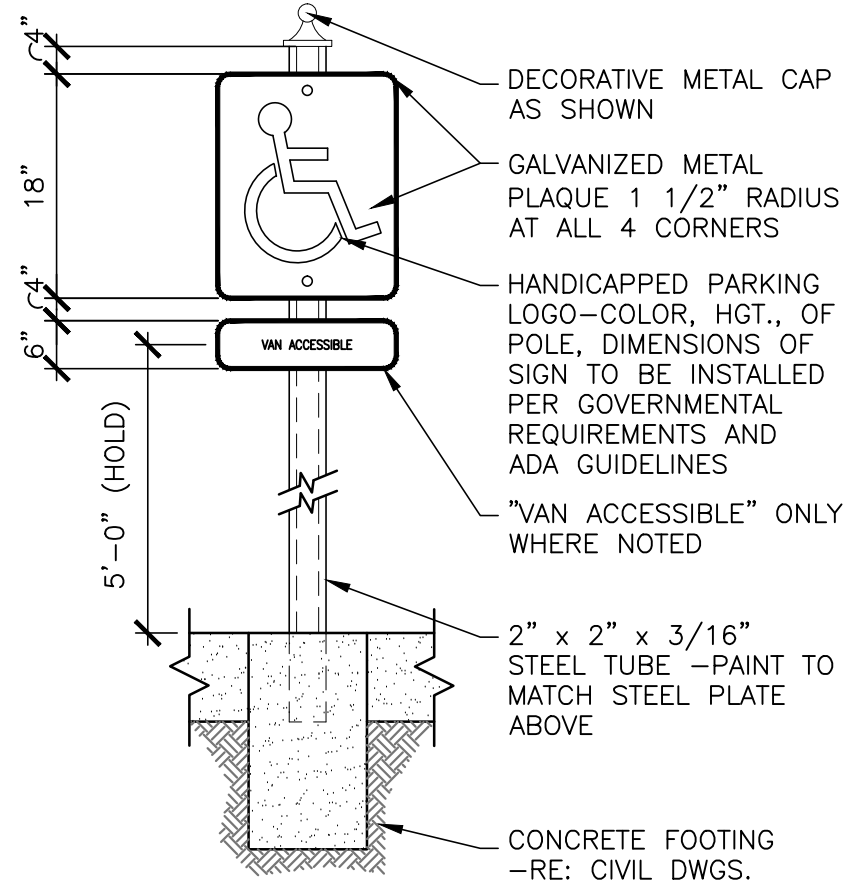
3 ACCESSIBLE SIGN DETAIL
