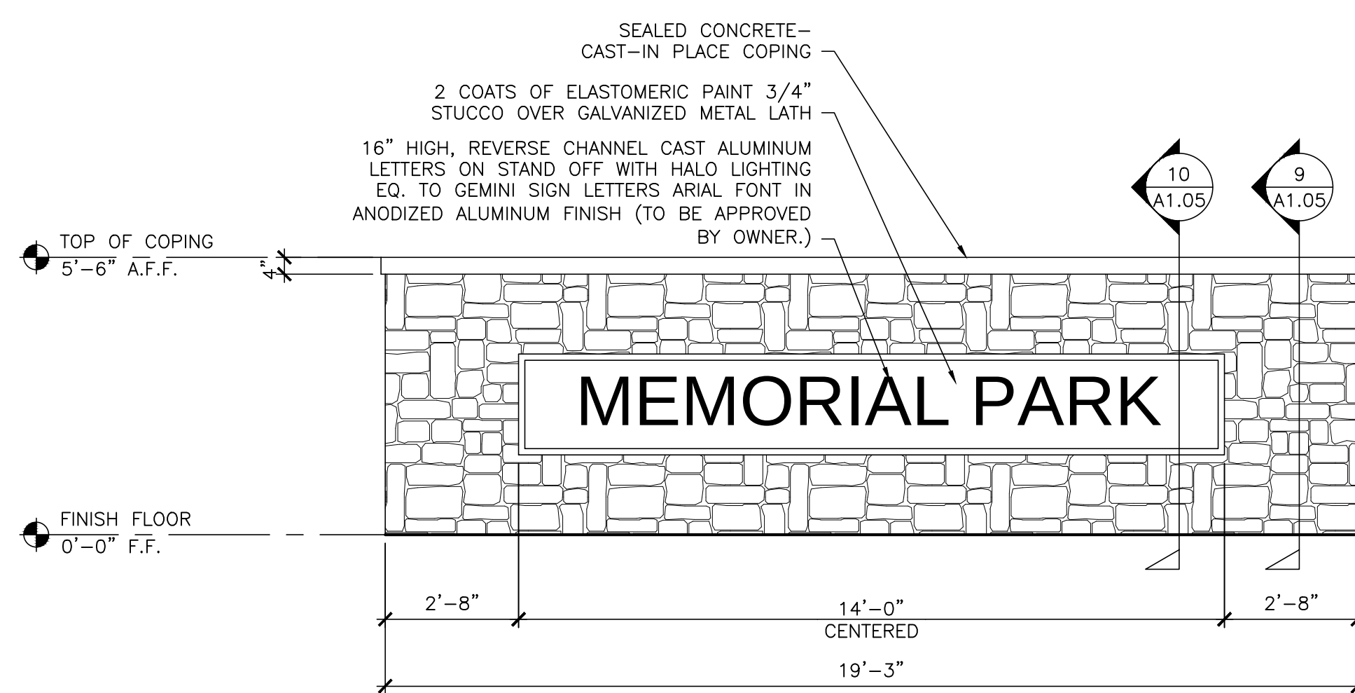
4 ALT. 2- MONUMENT SIGN ELEVATION SCALE: 3/8"=1'-0"
