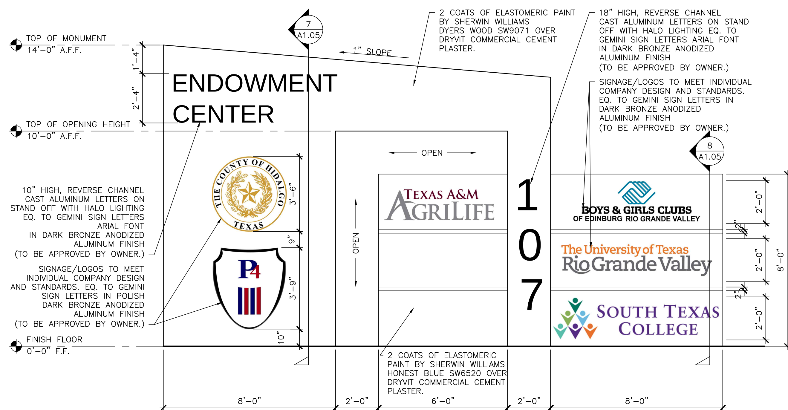
6 MONUMENT SIGN AT ENDOWMENT CENTER ELEVATION SCALE: 3/8"=1'-0"
