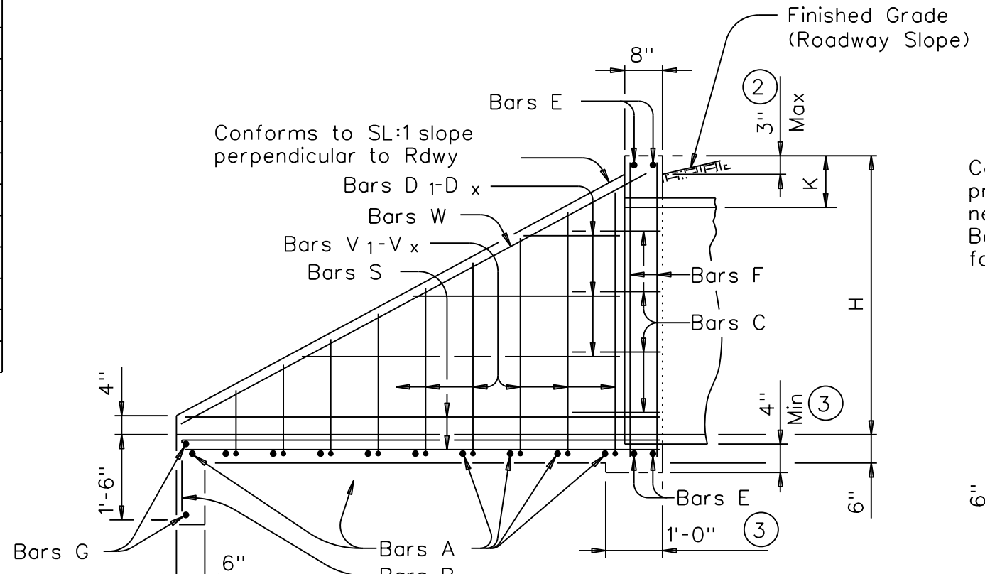
TYPICAL WING ELEVATION
