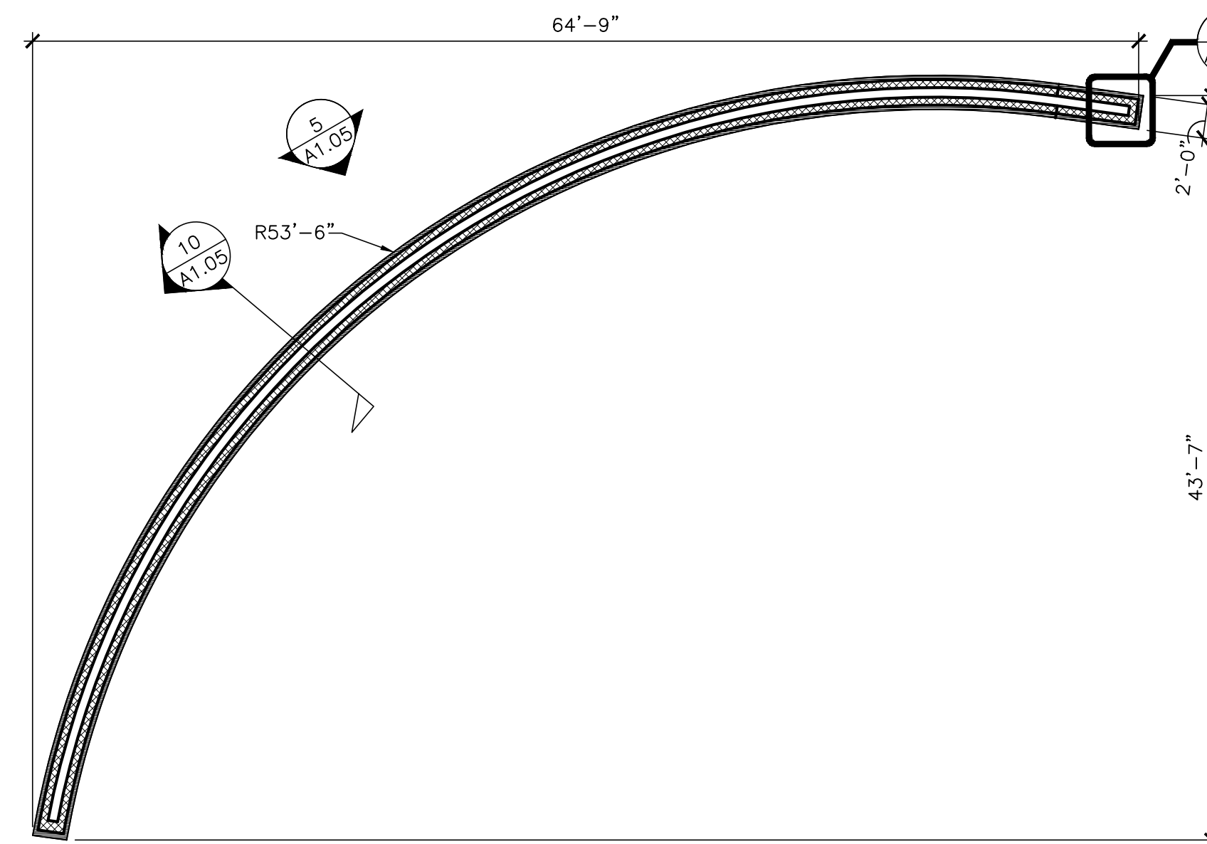
2 ALT. 2- PARTIAL SITE PLAN AT MONUMENT SCALE: 1/8"=1'-0"
