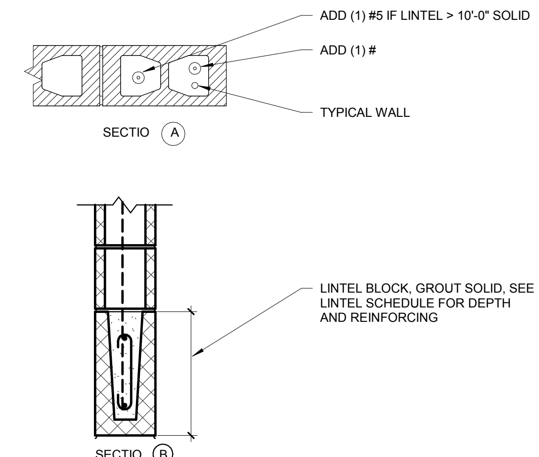
Typical CMU Lintel 1" = 1'-0"
