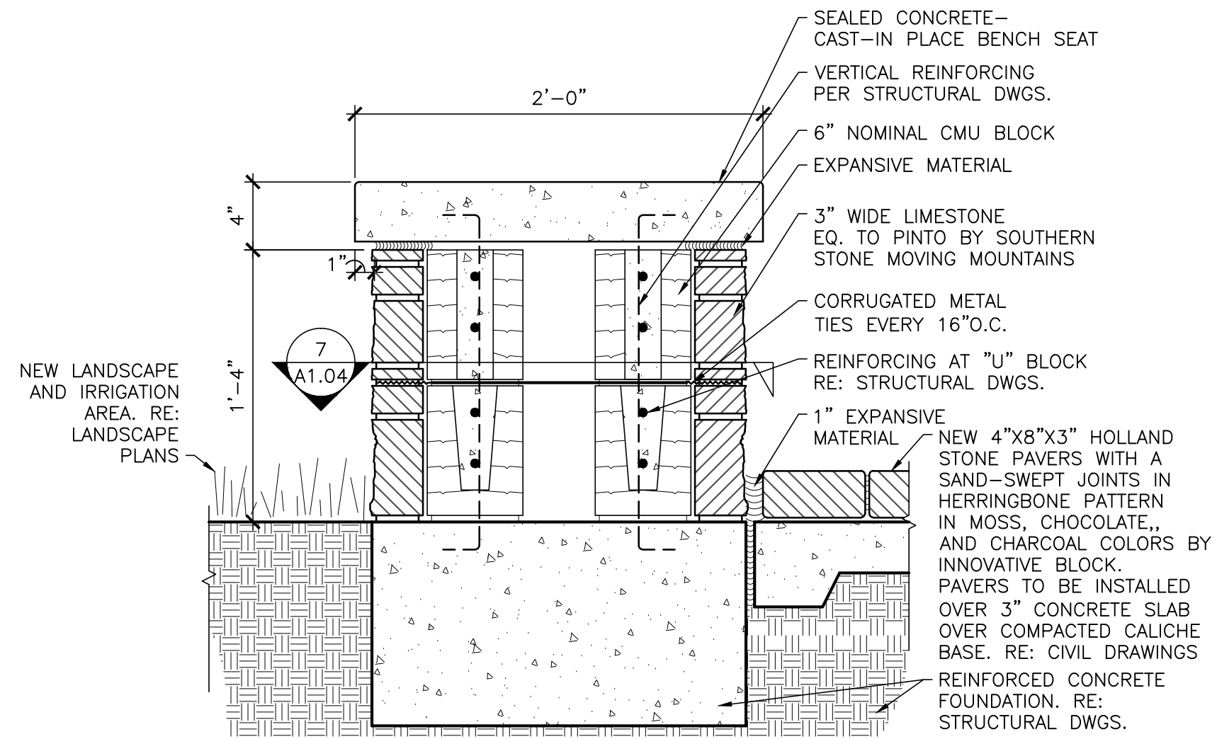
6 TREE WELL BENCH SECTION DETAIL SCALE: 1 1/2"=1'-0"
