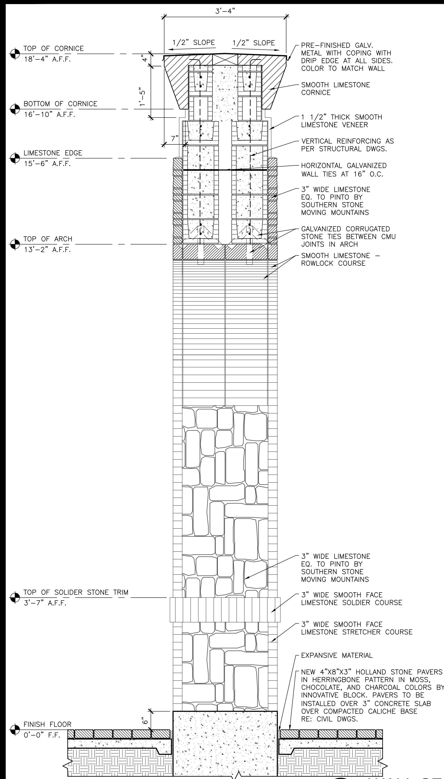
7 WALL SECTION SCALE: 3/4"=1'-0"
