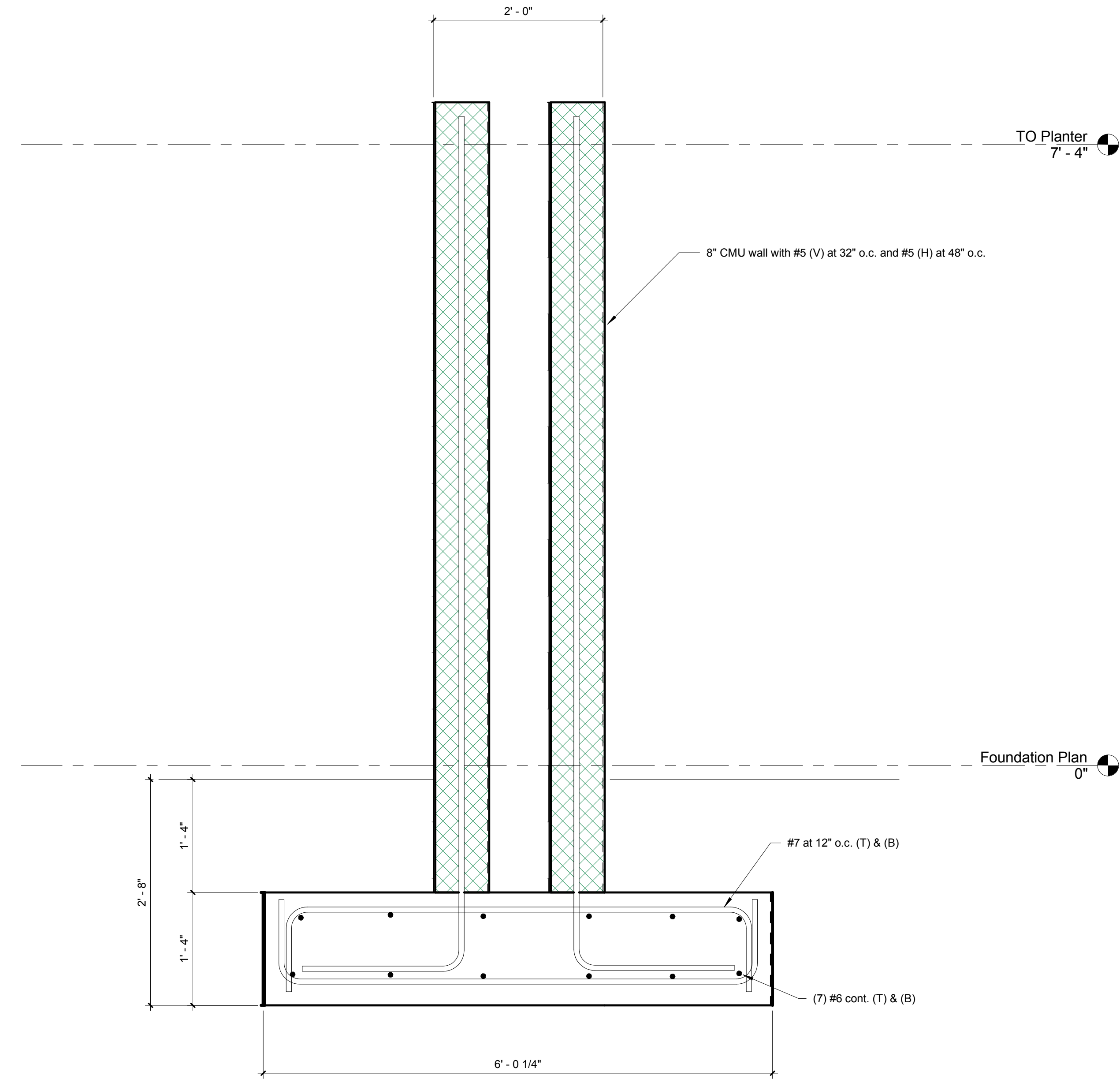
Detail 3 1" = 1'-0"
