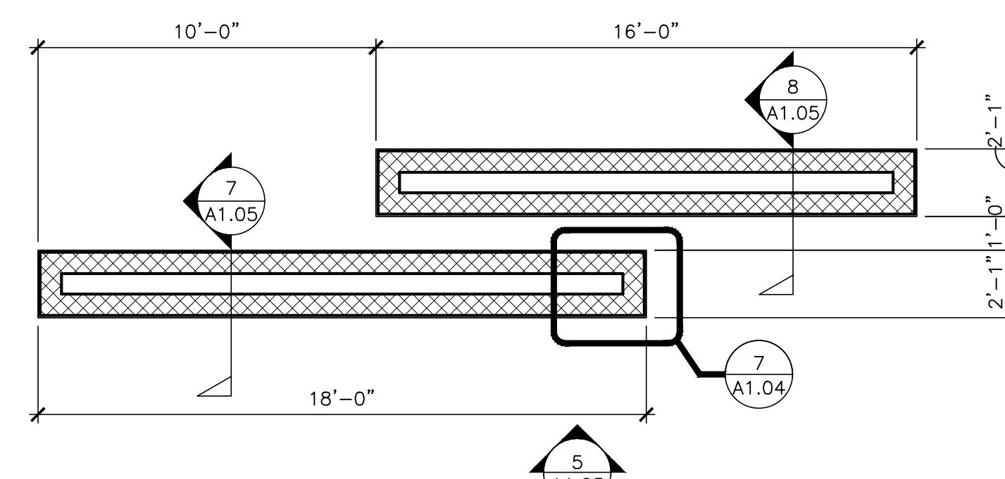
1 PARTIAL SITE PLAN AT MONUMENT SCALE: 1/4"=1'-0"
