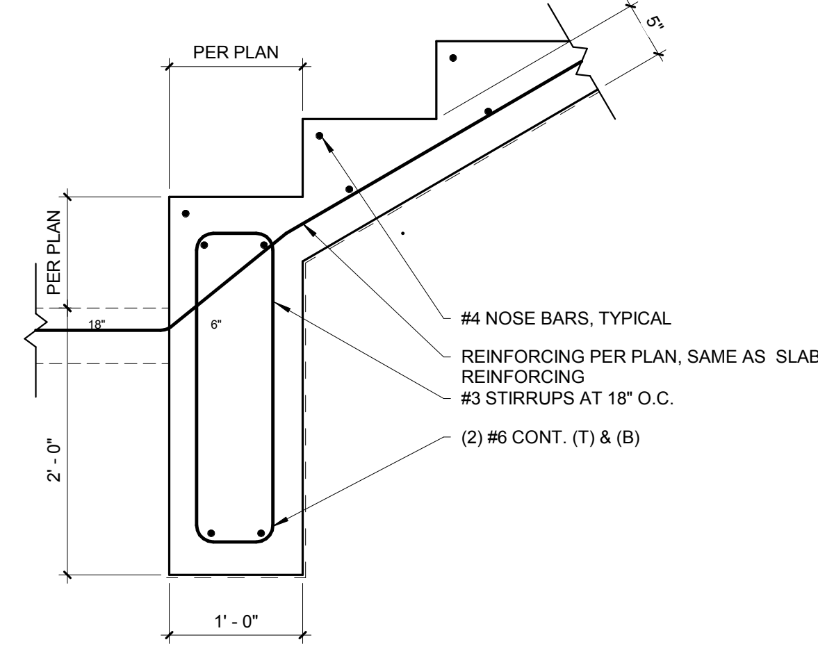
Footings at Concrete Steps, Exterior 1" = 1'-0"
