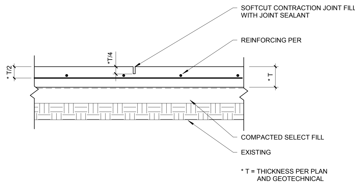
Typical Slab Construction Joint
