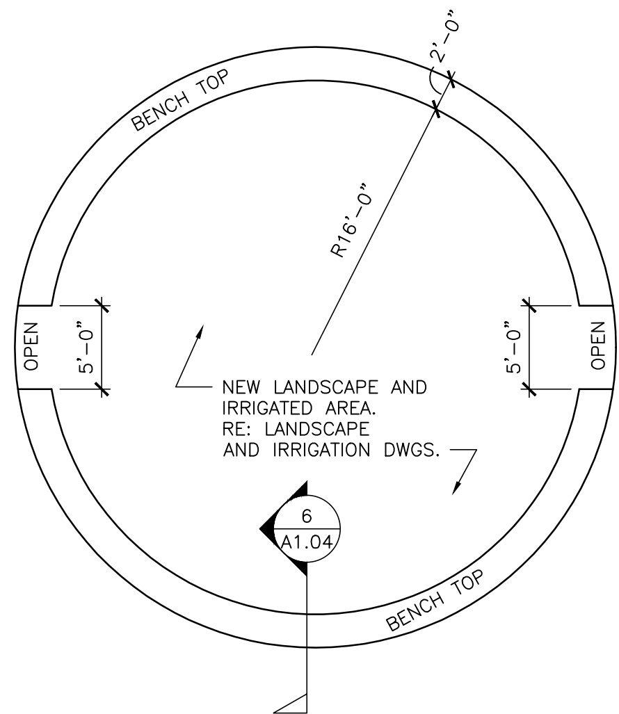
3 PARTIAL SITE PLAN AT "TREE WELL" BENCH FEATURE SCALE: 1/8"=1'-0"
