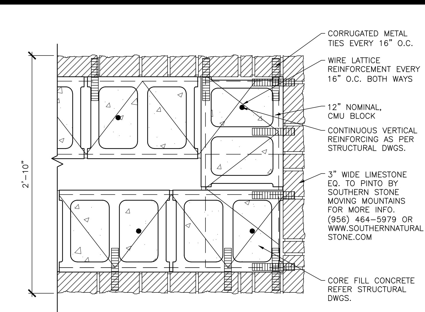
8 WALL DETAIL SCALE: 1 1/2"=1'-0"
