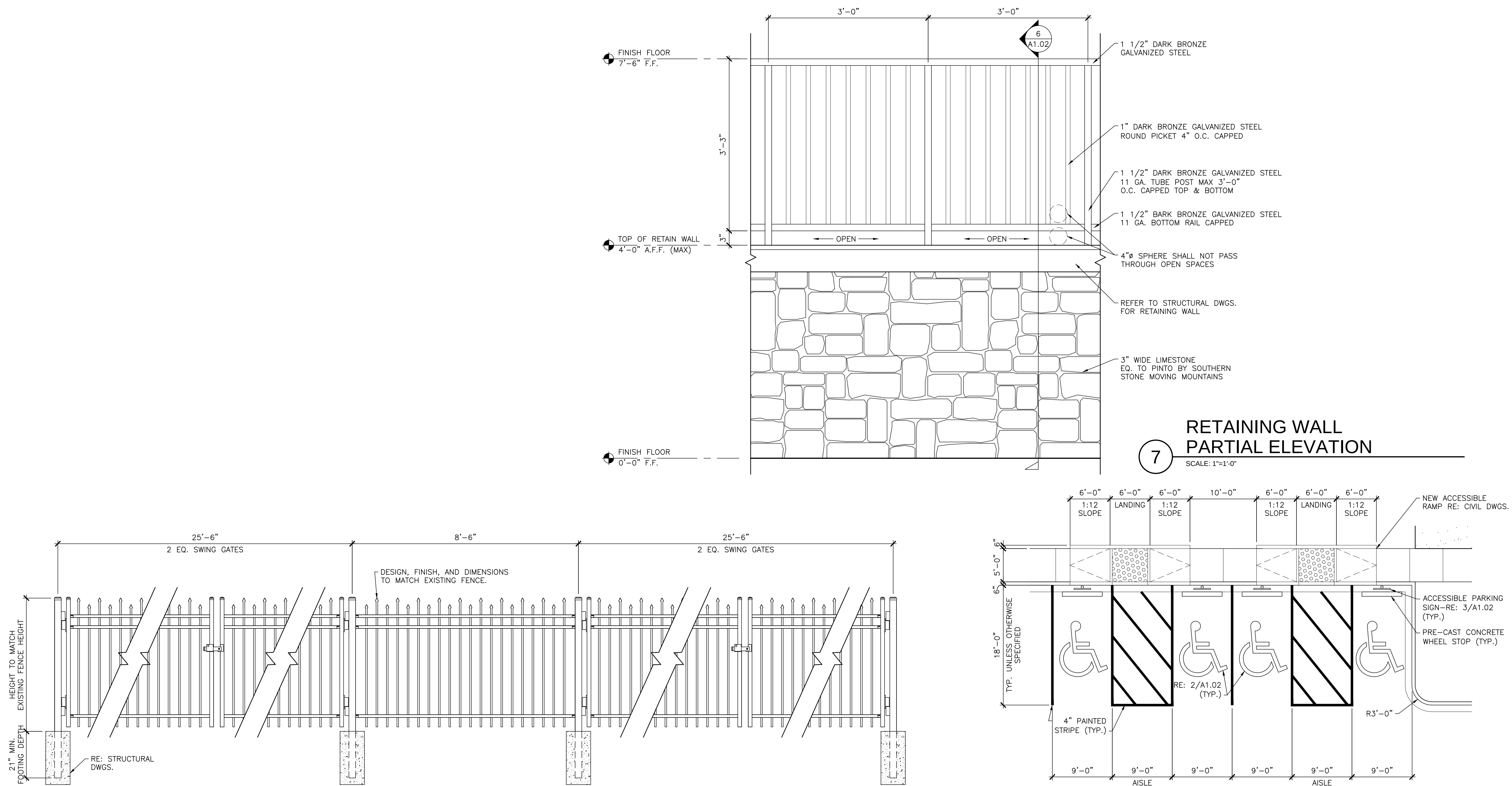
5 FENCE ELEVATION
