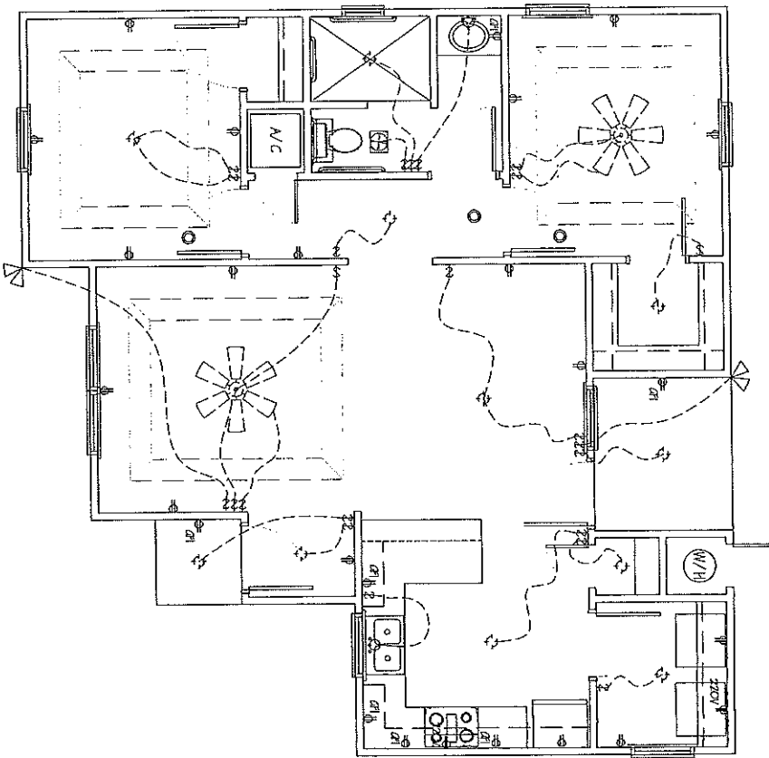
1 3/16" = 1'-0" ELECTRICAL PLAN
