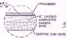
PARKING LOT SECTION N.T.S.
