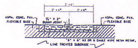
CONC. VALLEY GUTTER (TY\"A\") TO BE USED WHERE REQUIRED TO CARRY DRAINAGE WATER ACROSS STC STREETS N.T.S.
