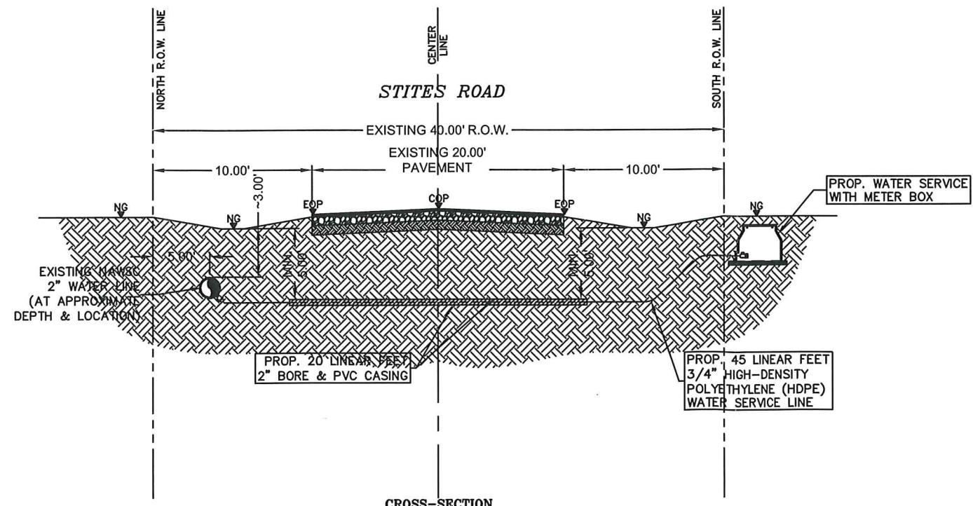
CROSS-SECTION SCALE: 1"=10'
