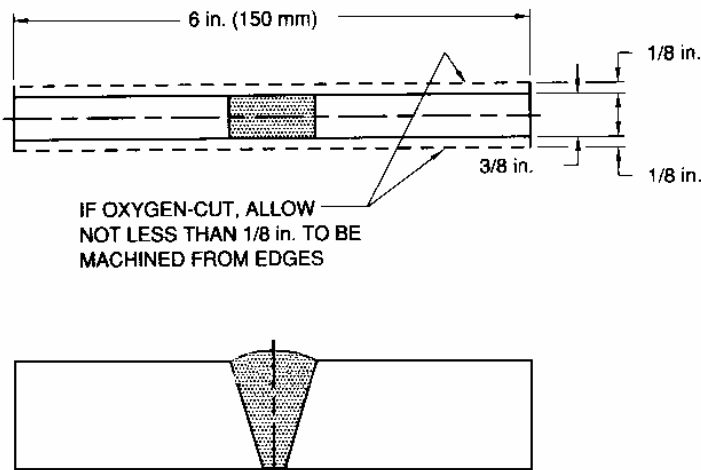
Figure 4 Side Bend Specimens
