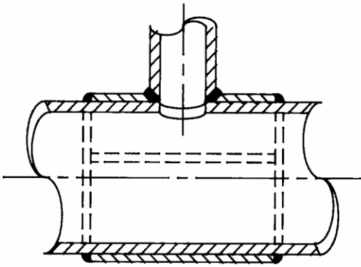
FULL ENCIRCLEMENT PAD (SLEEVE) TYPE
