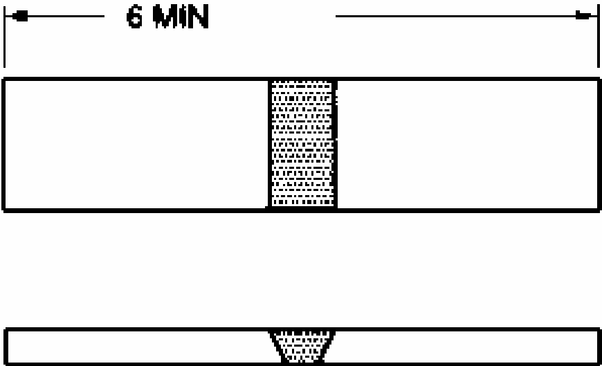
Figure 3 Root and Face Bend Specimens
