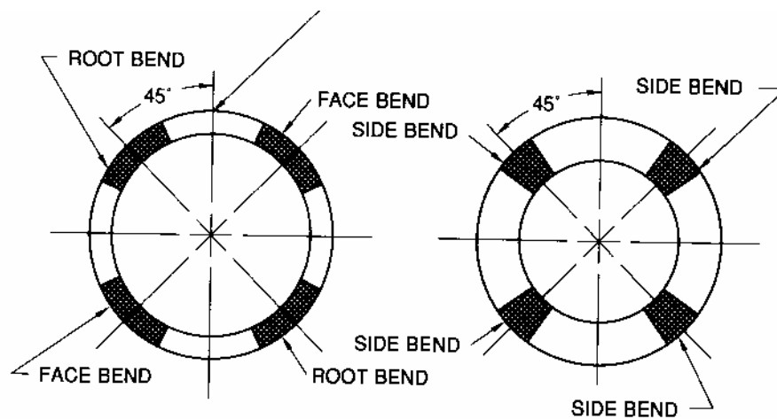
Figure 2 Pipe Test Specimen Location
