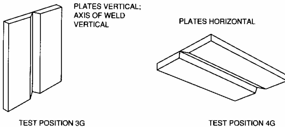
Figure 6 Plate Test Positions
