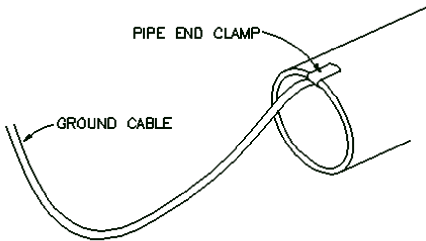
FIGURE 2 PROCEDURE - POTENTIAL MEASUREMENTS OF PIPE
