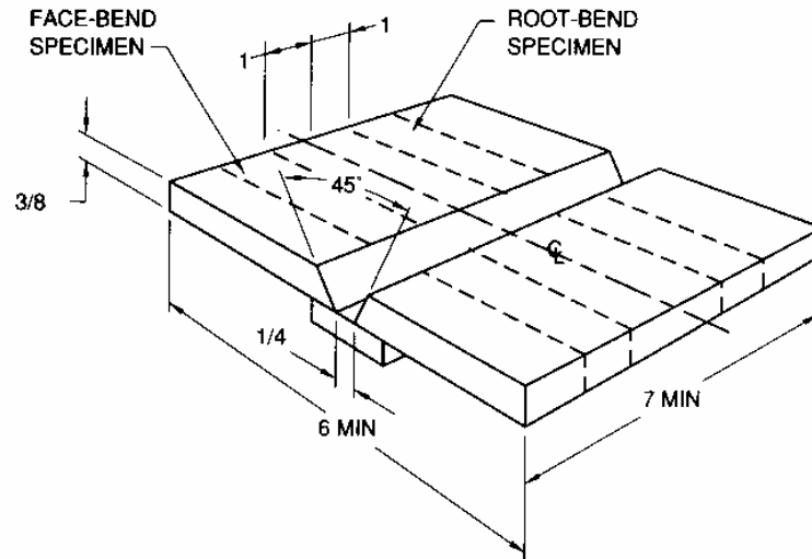
Figure 5 Plate Test Weld and Specimen Location
