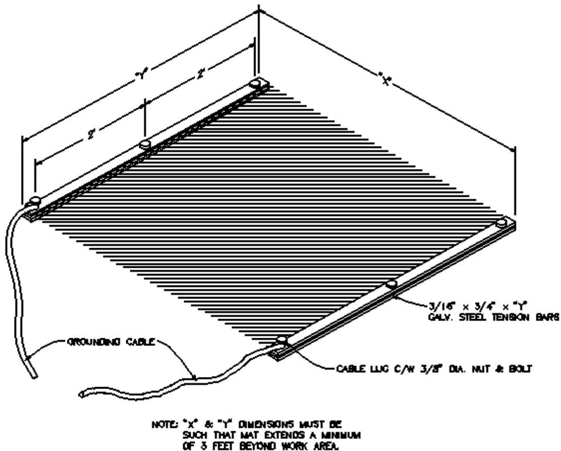
FIGURE 5 PROCEDURE - TEMPORARY GRADIENT CONTROL MATS
