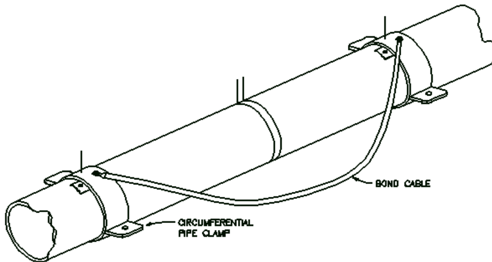
FIGURE 4 PROCEDURE - BONDING & PIPING AT TIE-INS & CUTOUTS
