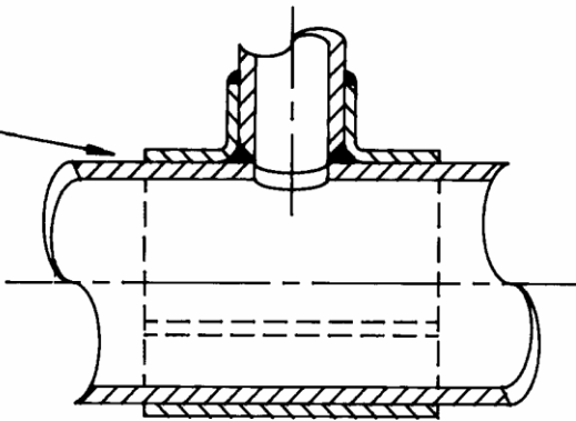
FULL ENCIRCLEMENT SADDLE TYPE
