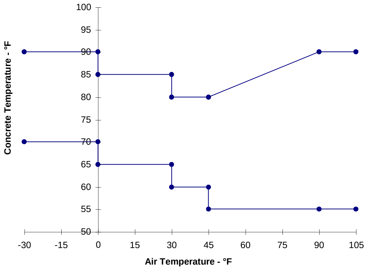
FIGURE 1 Concrete Temperature Limitations at Time of Placement
