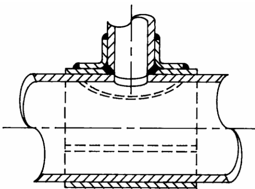
SADDLE AND FULL ENCIRCLEMENT PAD (SLEEVE) TYPE
