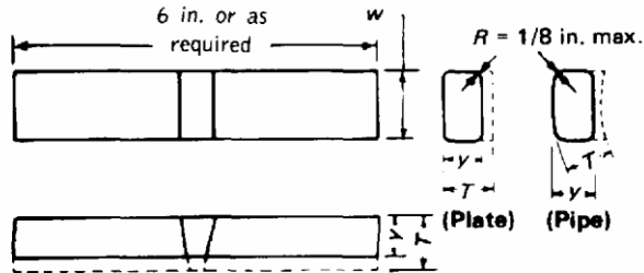
Face-bend specimen
