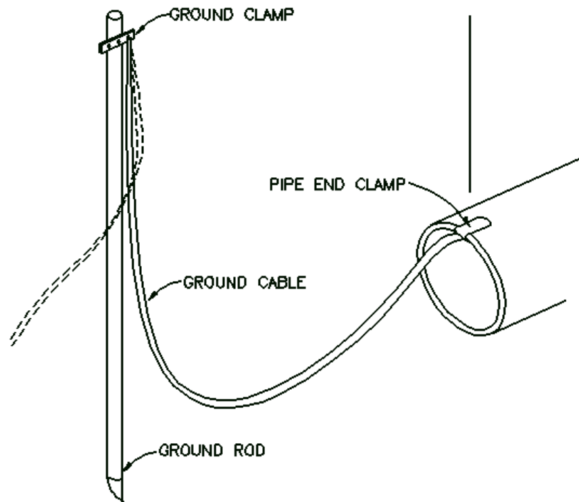
FIGURE 3 PROCEDURE - CONNECTING & DISCONNECTING GROUNDING FACILITIES
