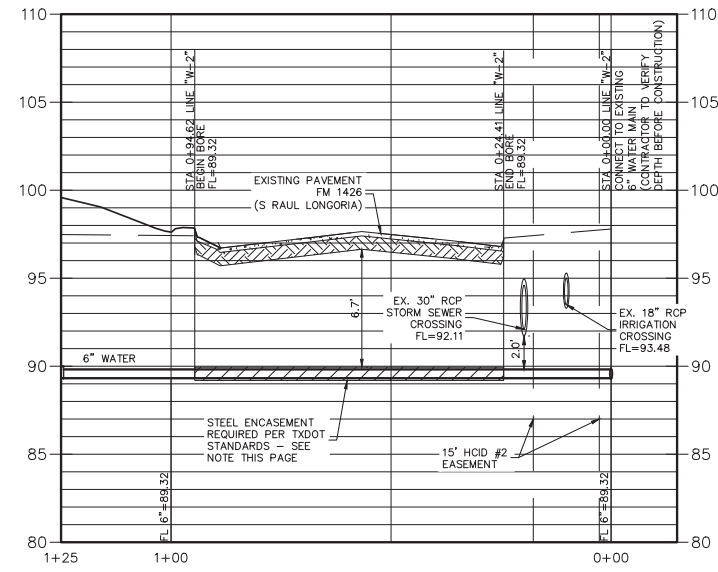
WATER LINE "W-2" H: 1"=40' V: 1"=10'
