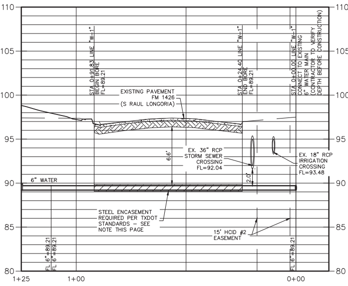
WATER LINE "W-1" H: 1"=40' V: 1"=10'
