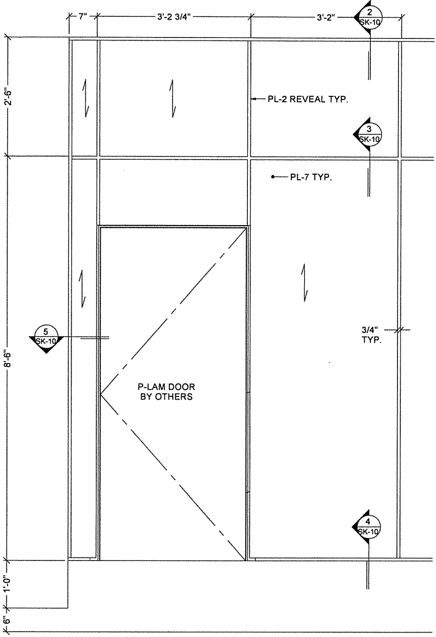
1 ELEVATION SK-10 SCALE: 1/2"=1'-0" REF ARCHIT: 3/A-254
