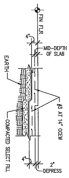
C-SHOWER DEPRESS
