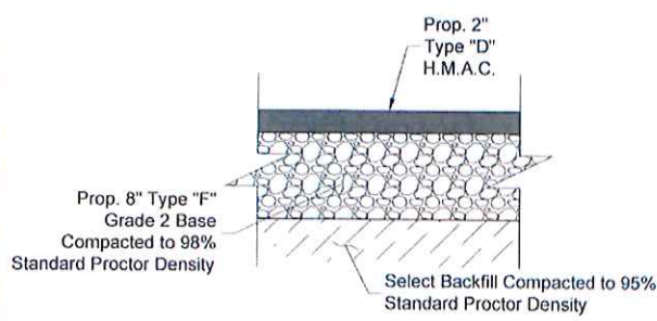
Mile 8 1/2 Roadway Paving Detail SCALE: 1"=1'-0"
