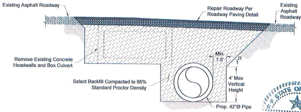
Mile 8 1/2 Roadway Backfill Detail SCALE: 1"=4'-0"
