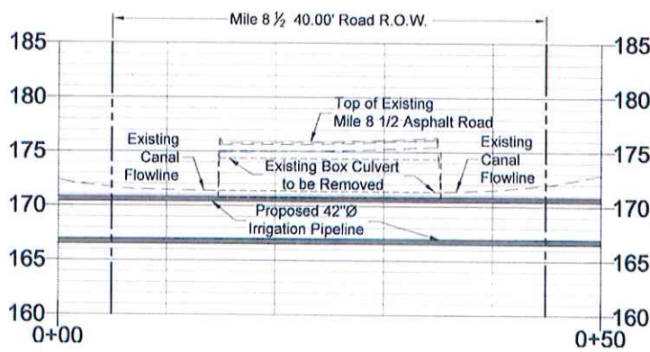
Profile Mile 8 1/2 Proposed Irrigation Line Road Crossing Horizontal: 1"=10' Vertical: 1"=10'
