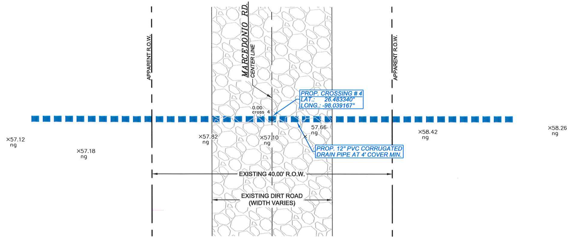
PLAN VIEW SCALE: 1"=10'
