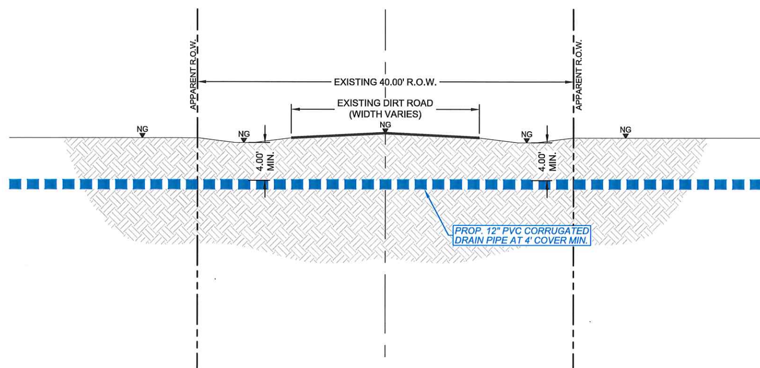
MARCEDONIO RD. CROSS-SECTION VIEW SCALE: 1"=10'
