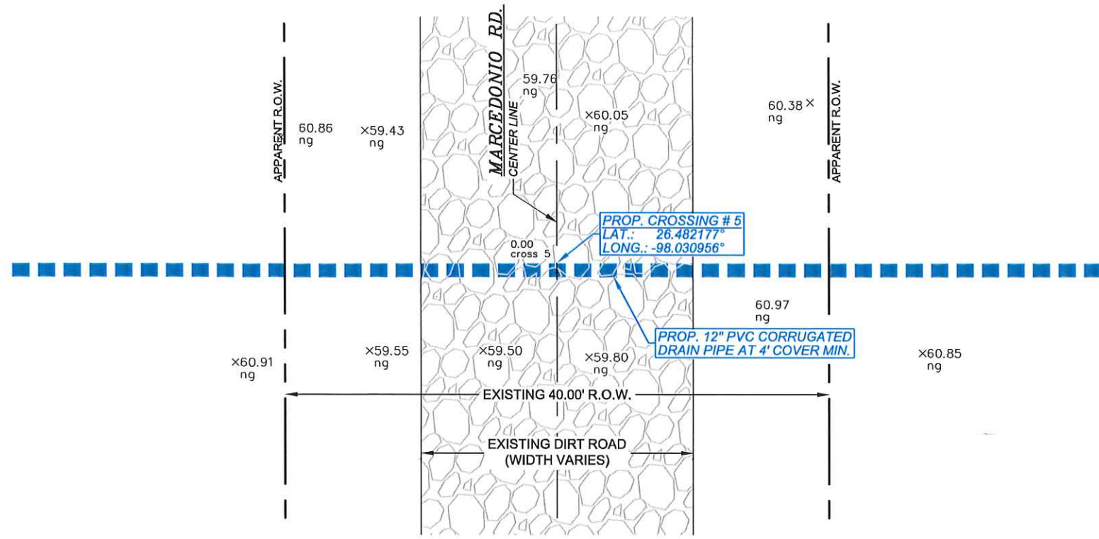
PLAN VIEW SCALE: 1"=10'
