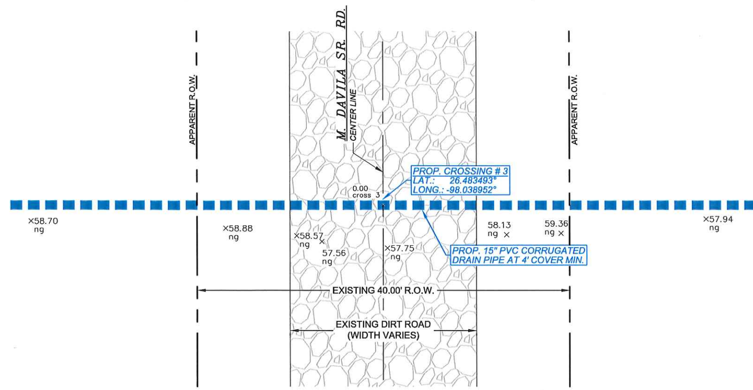
PLAN VIEW SCALE: 1"=10'
