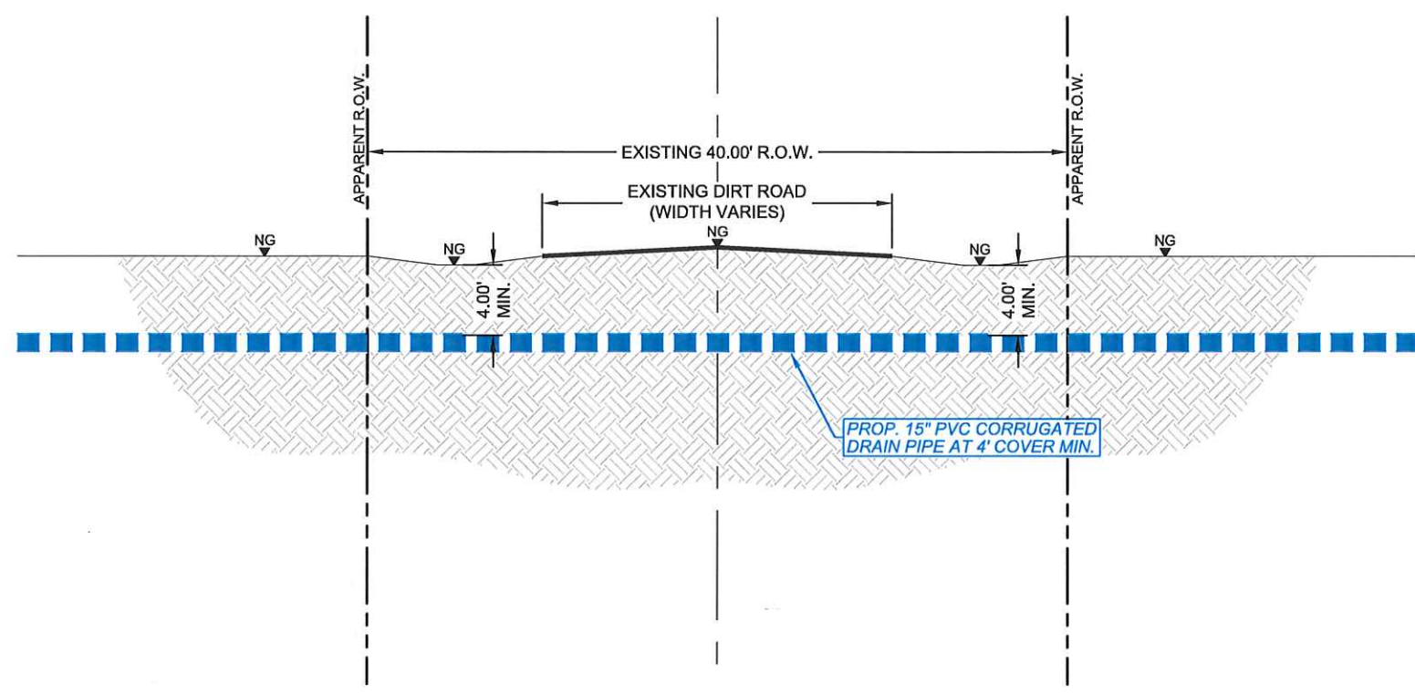
M. DAVILA SR. RD. CROSS-SECTION VIEW SCALE: 1"=10'
