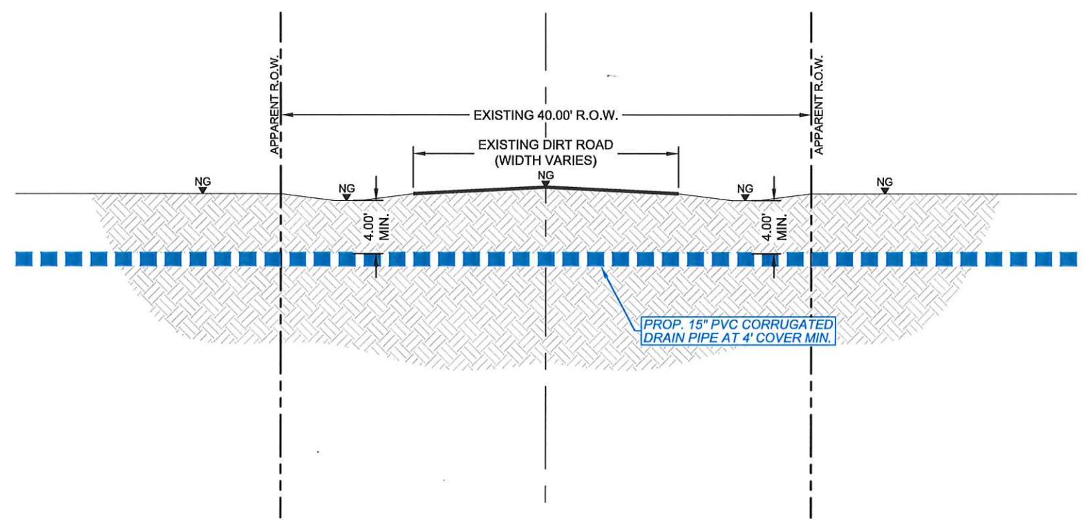
"UNNAMED" RD. CROSS-SECTION VIEW SCALE: 1"=10'
