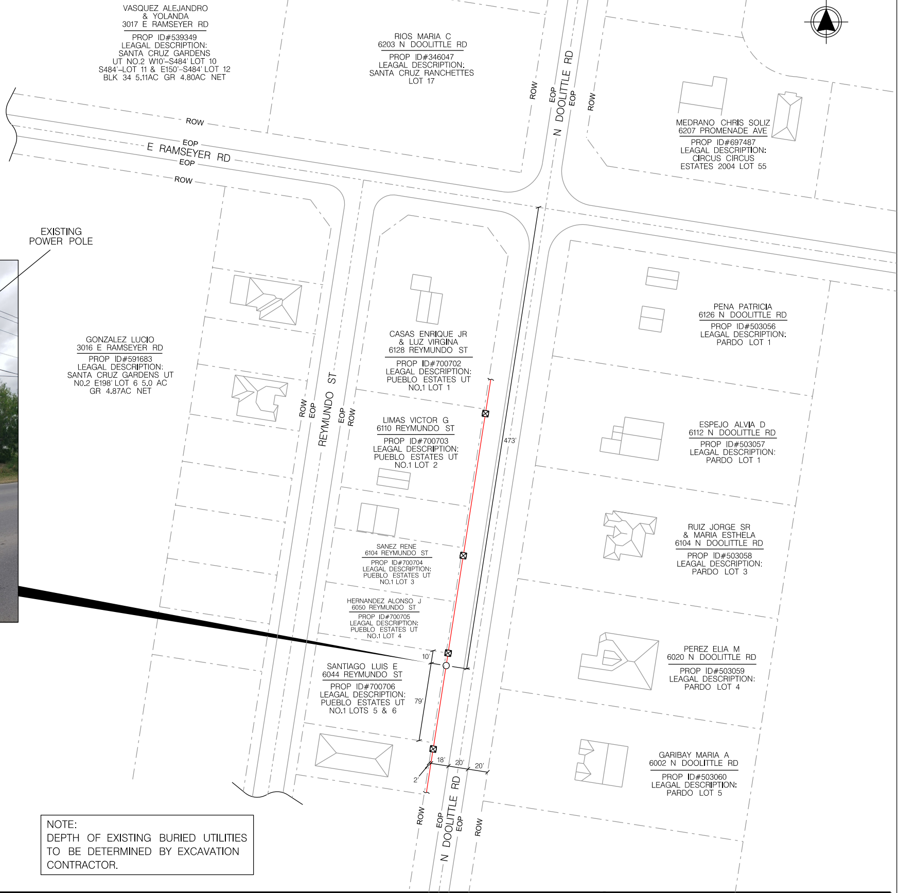
LAT: 26.300420 - LONG: -98.118389 NEW PROPOSED SPECTRUM POLE 2' IN ROW & 18' FROM EOP
