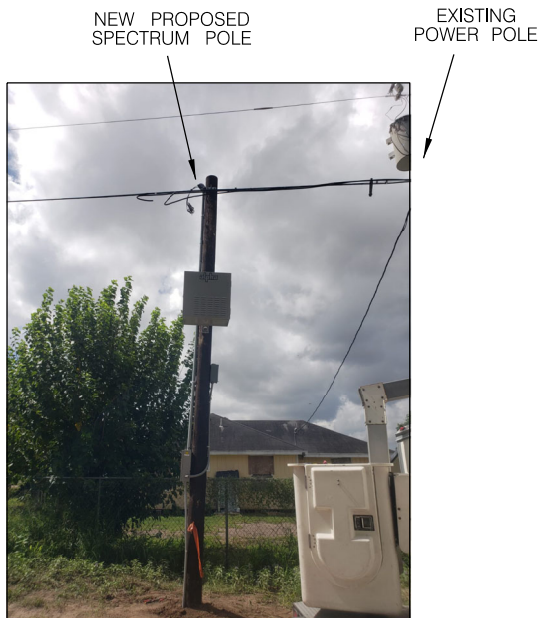
LAT: 26.263694 LONG: -98.044027 NEW PROPOSED SPECTRUM POLE 2' IN ROW & 14' FROM EOP
