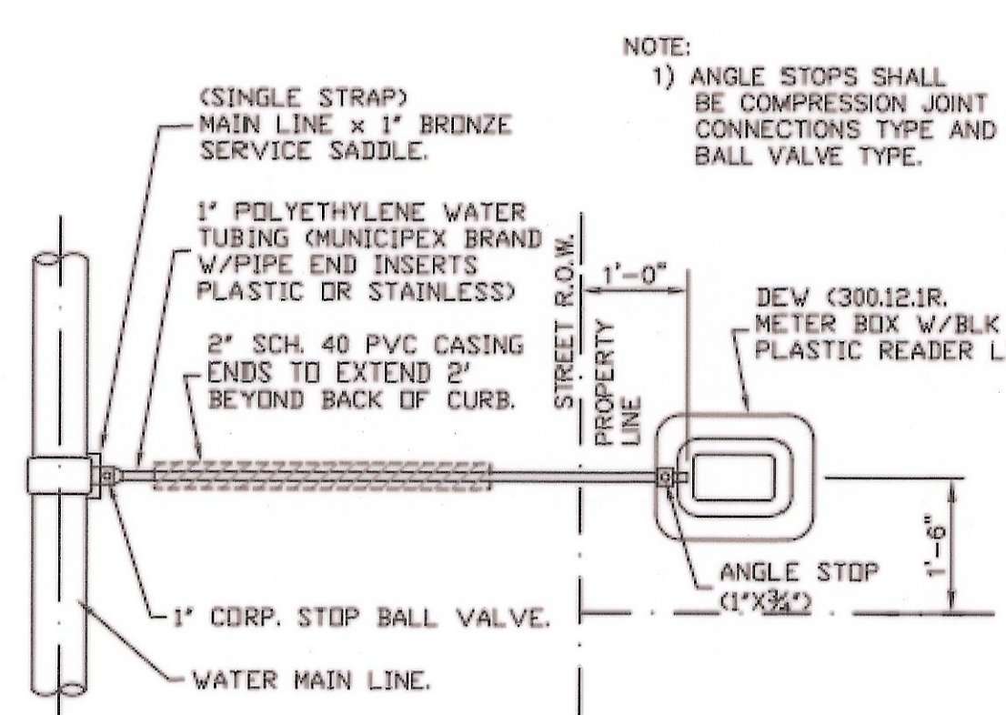
SINGLE WATER SERVICE CONNECTION DETAIL NTS
