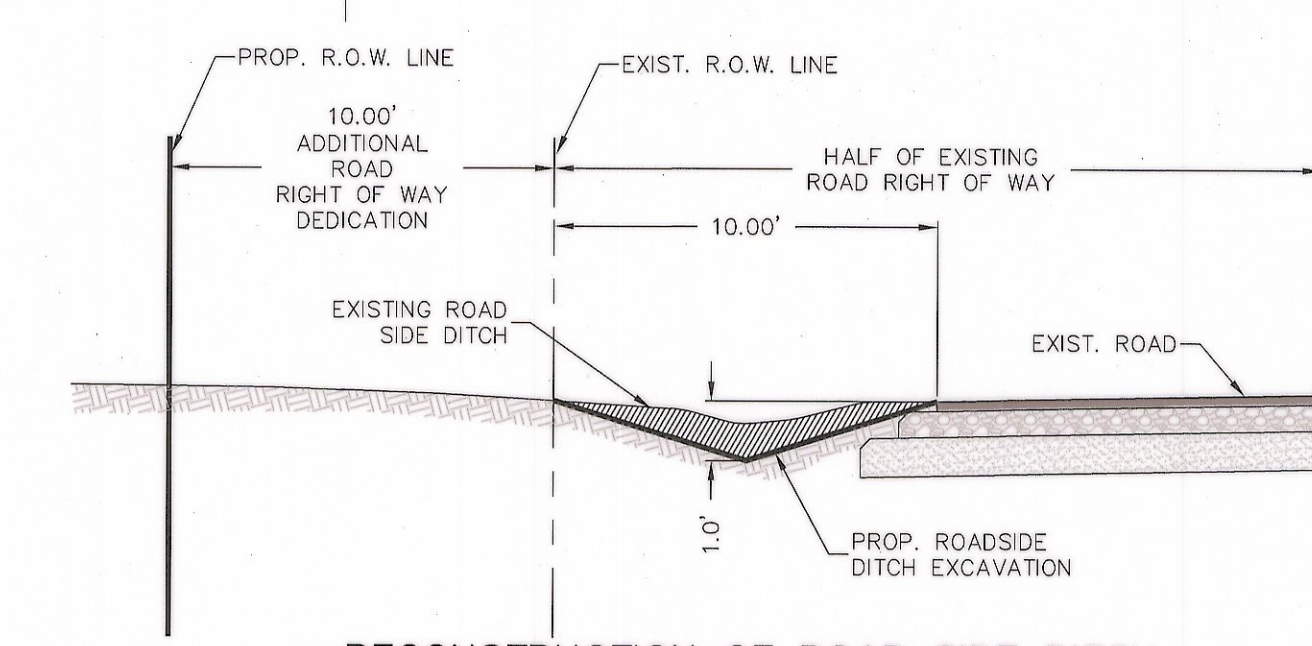
RECONSTRUCTION OF ROAD SIDE DITCH NTS RE-GRADING 1,500 LF OF EXISTING ROADSIDE DITCH TO PROVIDE A 10-FOOT WIDE x 1 FOOT DEEP "V" SHAPE ROADSIDE DITCH WILL PROVIDE APPROXIMATELY 7,500 CUBIC FEET OF STORAGE VOLUME. THE REQUIRED STORAGE VOLUME FOR THIS SUBDIVISION IS 6,366 CUBIC FEET THEREFORE, THE STORAGE VOLUME REQUIREMENTS ARE MET.
