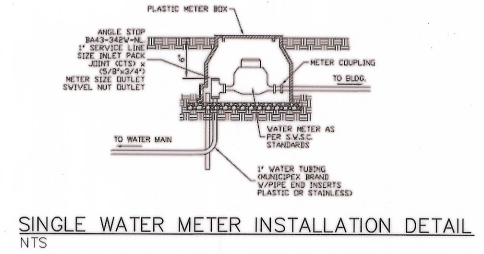
SINGLE WATER METER INSTALLATION DETAIL NTS
