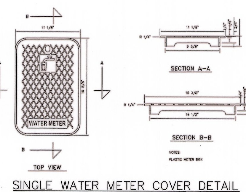
SINGLE WATER METER COVER DETAIL NTS
