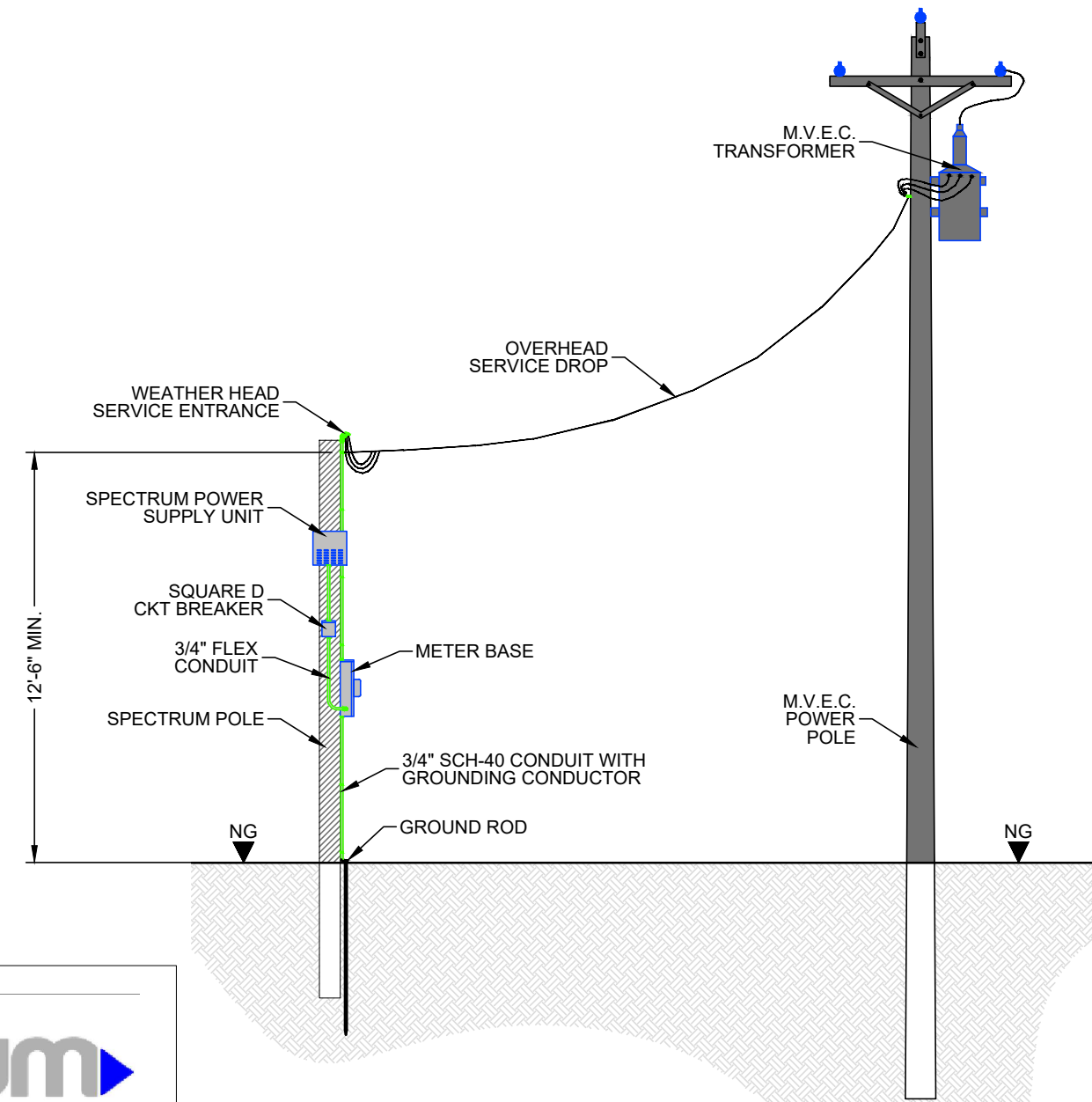
DETAIL "A" (CROSS-SECTION VIEW) NOT TO SCALE
