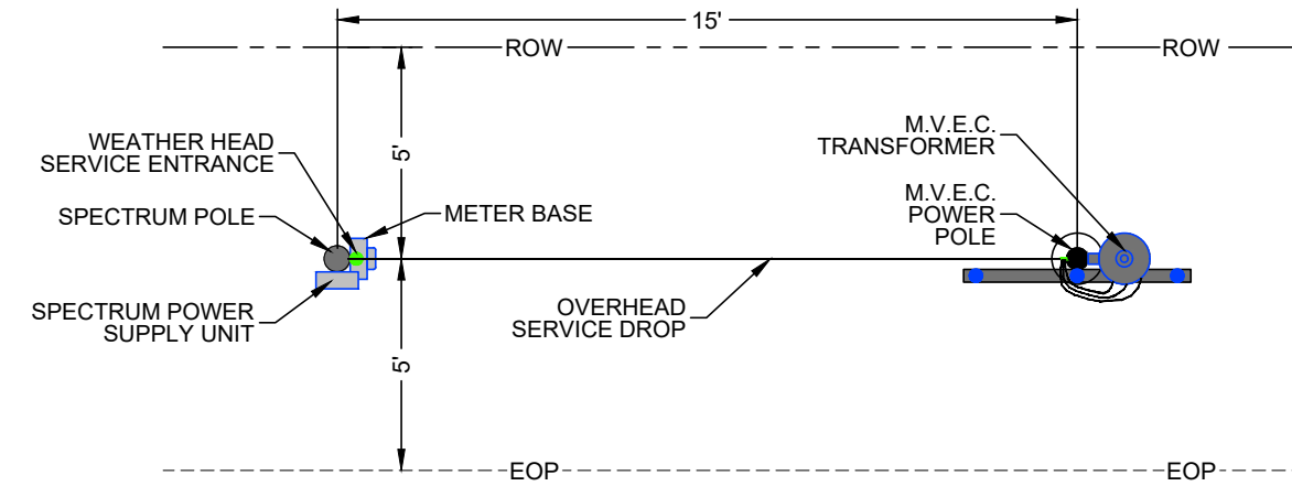
DETAIL "A" (PLAN VIEW) NOT TO SCALE
