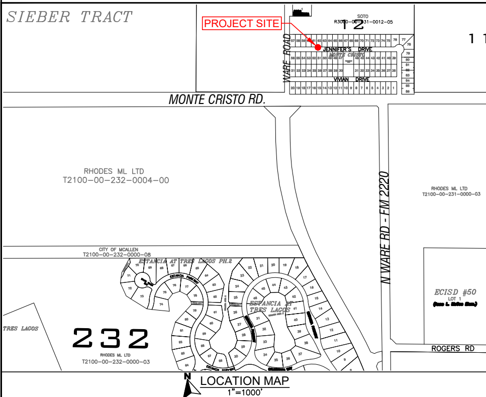
LAT: 26.351600° - LONG: -98.245495° NEW SPECTRUM POLE MOUNTED POWER SUPPLY 2' SOUTH FROM ROW & 12' NORTH FROM EOP
