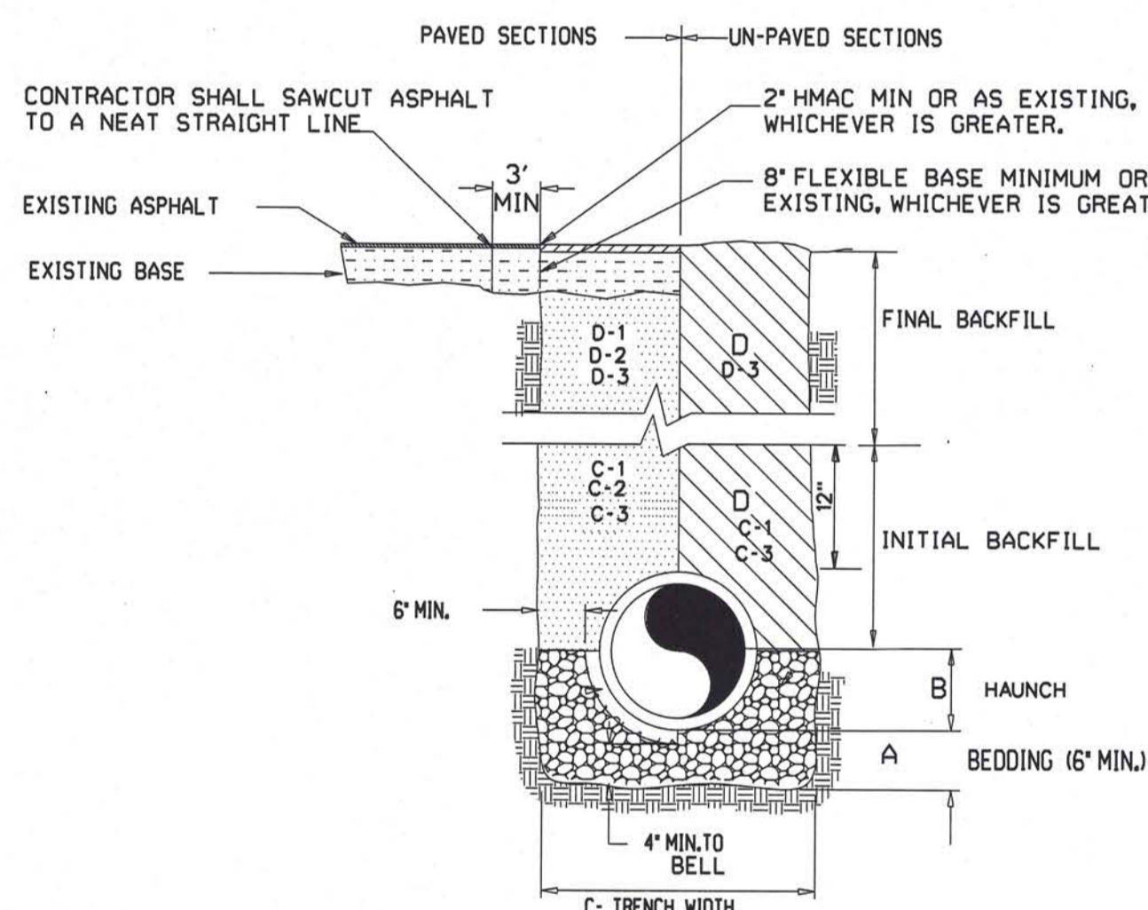
STORM TRENCH BEDDING AND BACKFILL DETAILS
