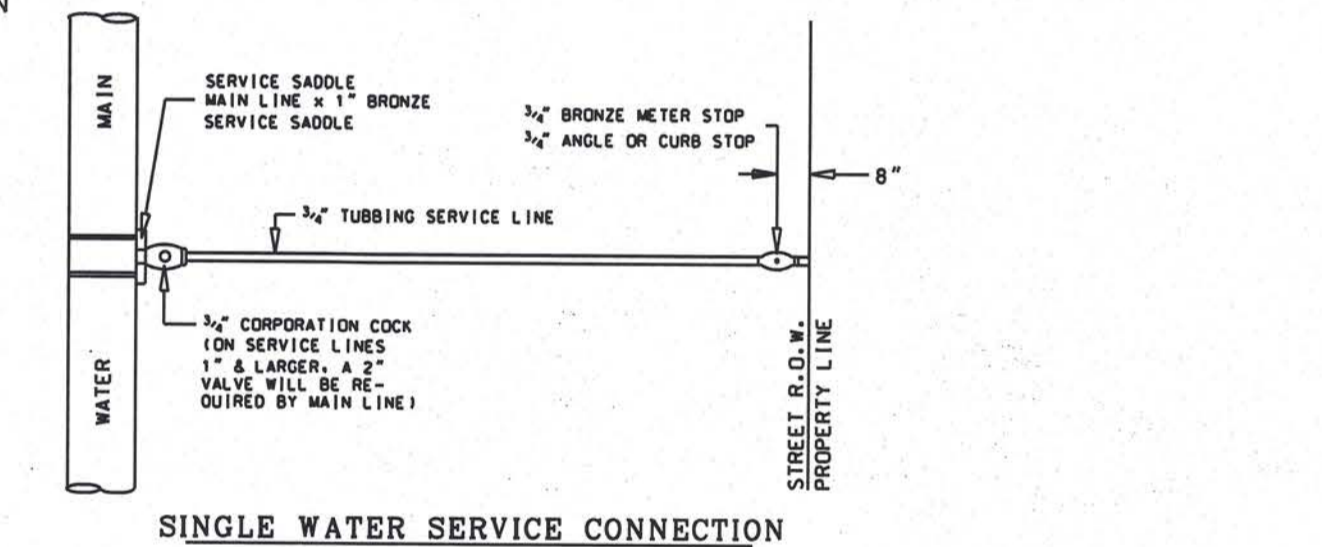
SINGLE WATER SERVICE CONNECTION
