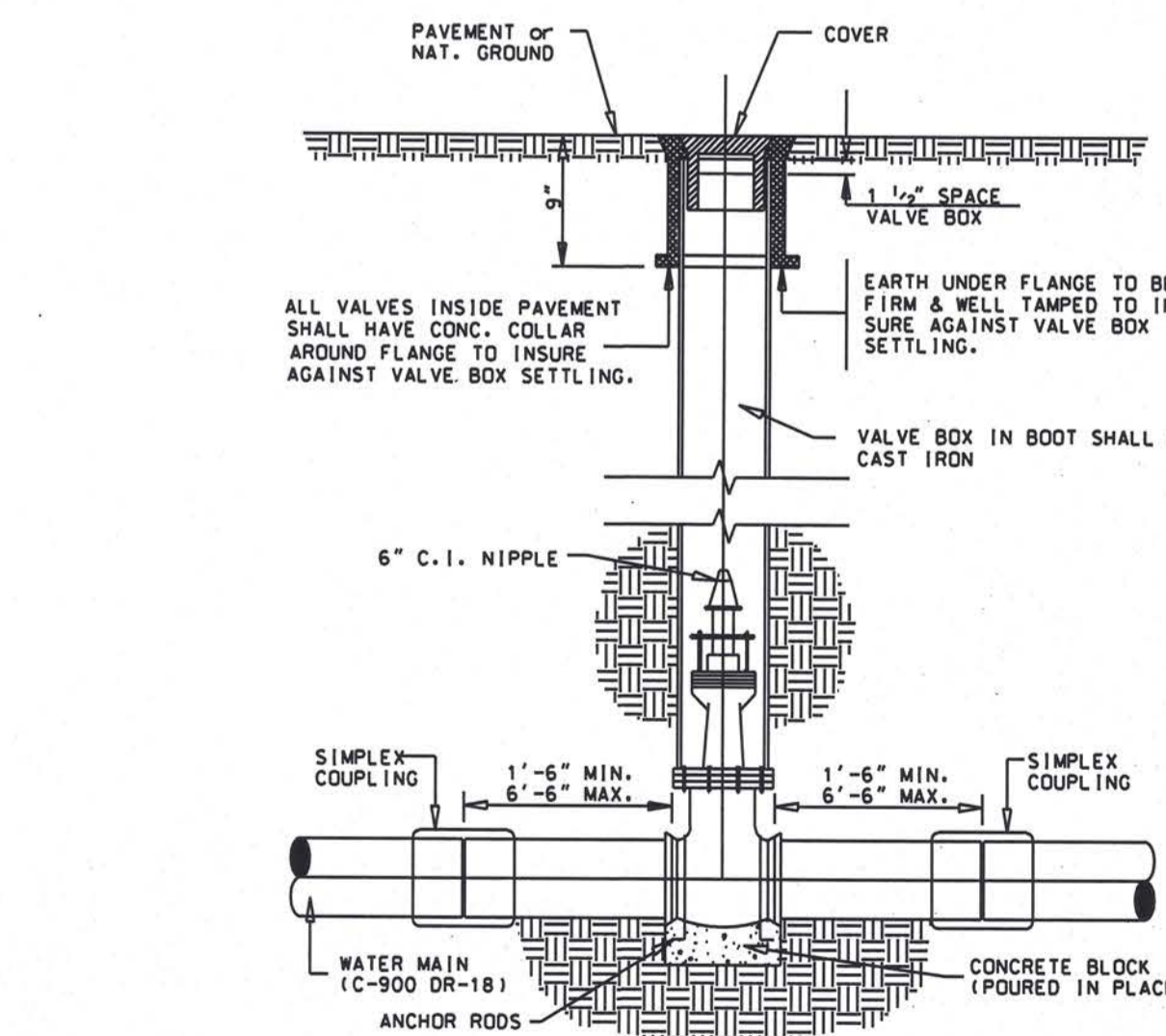
TYPICAL VALVE and VALVE BOX INSTALLATION
