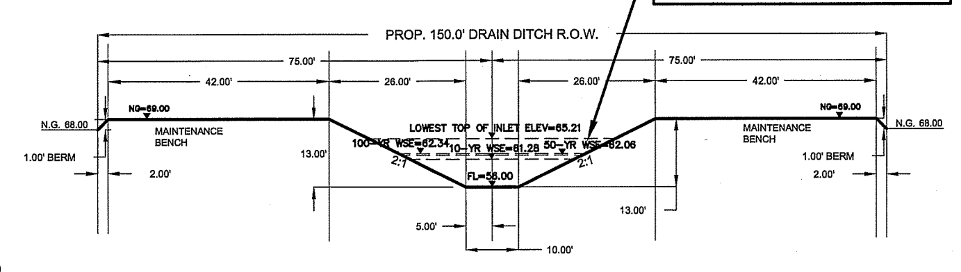
SECTION C-C PROPOSED DRAINAGE DITCH CROSS SECTION
