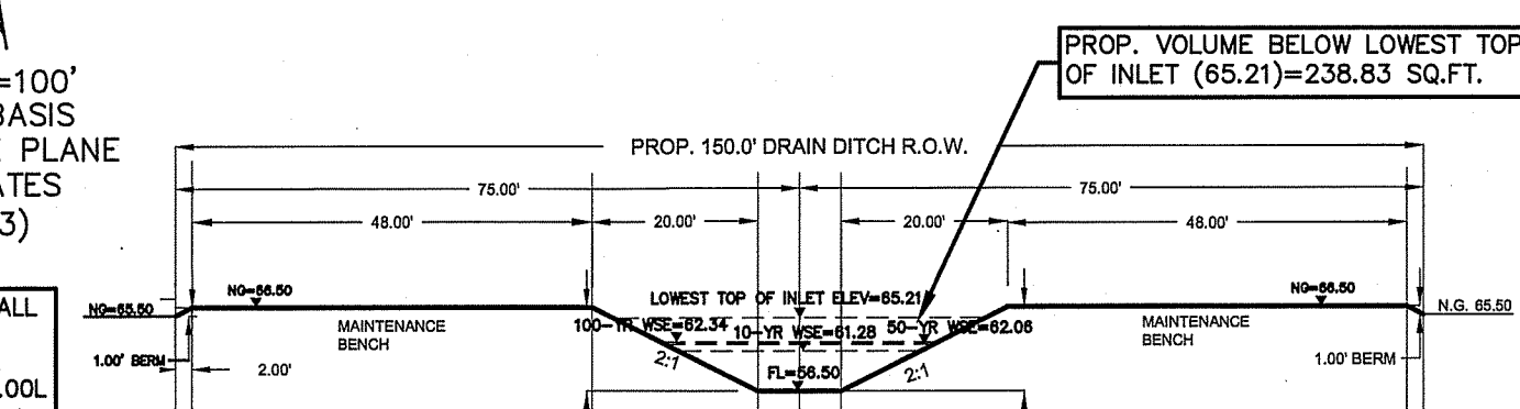
SECTION D-D PROPOSED DRAINAGE DITCH CROSS SECTION
