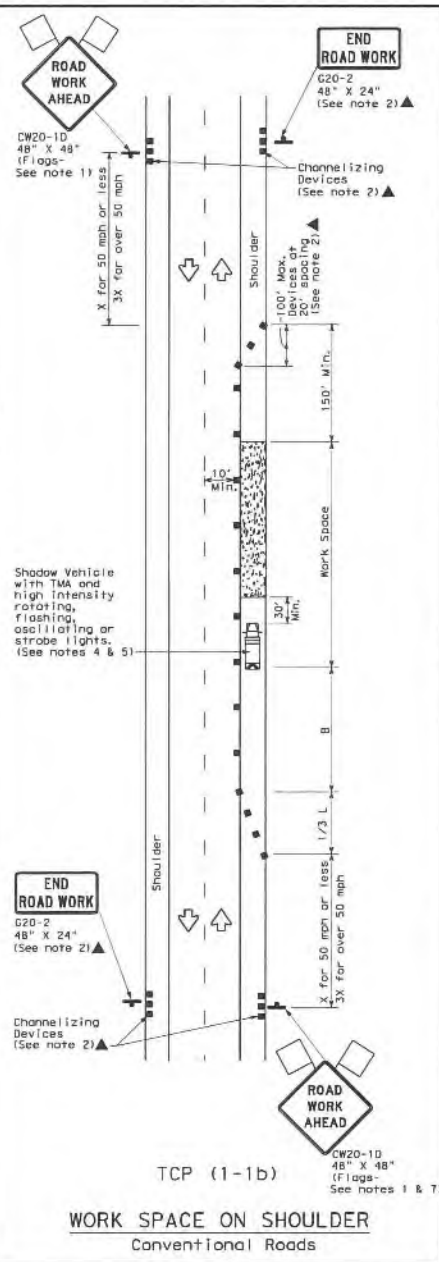
WORK SPACE NEAR SHOULDER Conventional Roads
