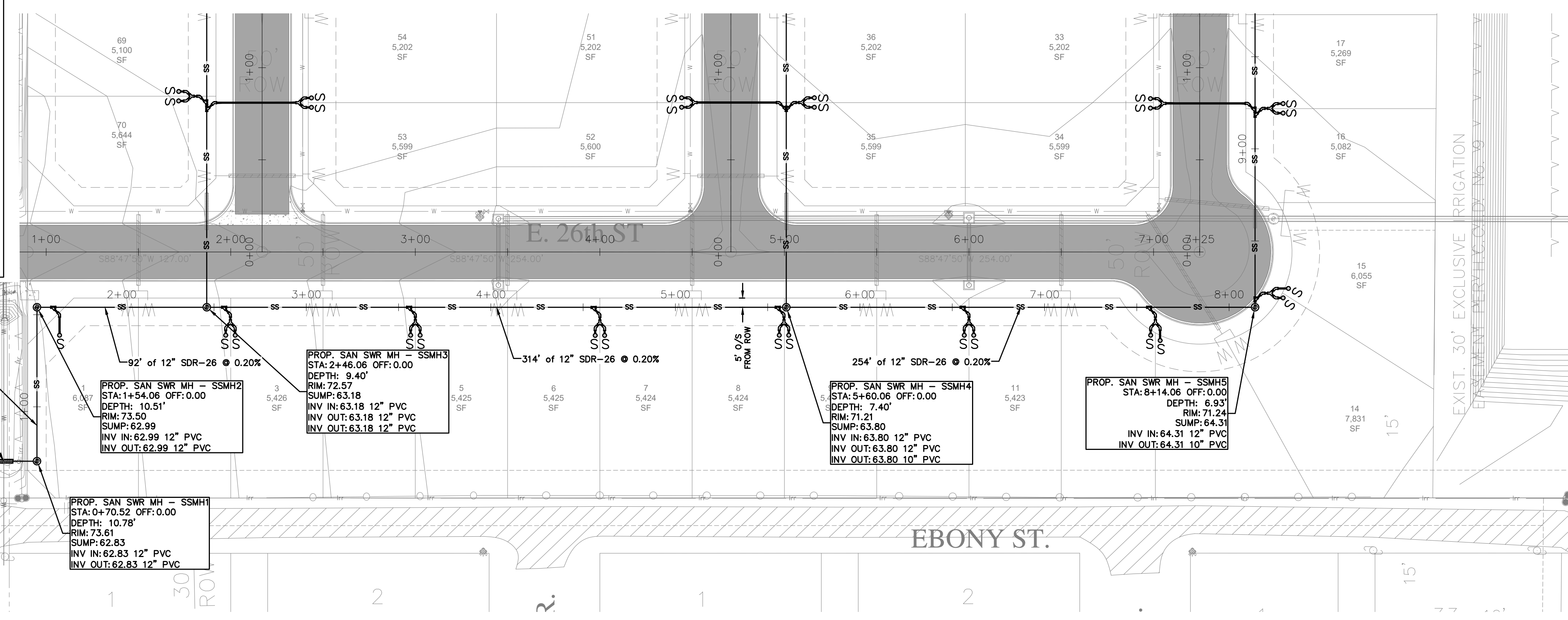
SANITARY SEWER PLAN (SSMH0-SSMH5)
