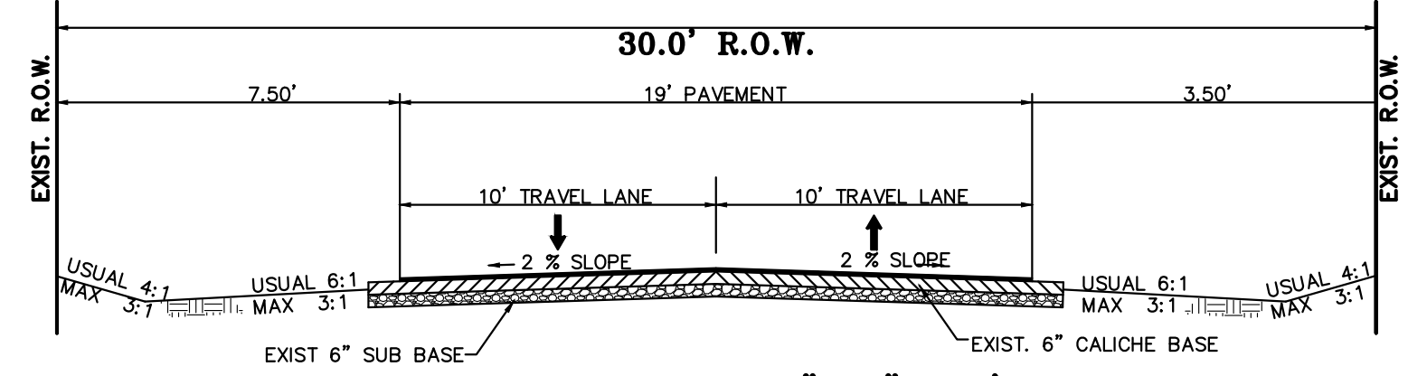
EXIST TYPICAL SECTION ON "C-C" 30.0' R.O.W. (N.T.S.)
