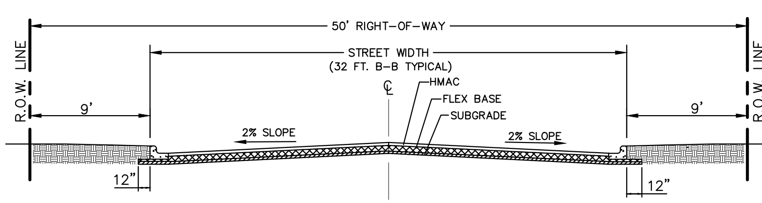
TYPICAL LOCAL STREET CROSS-SECTION "B-B" NOT TO SCALE
