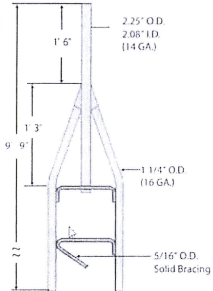
STANDARD TOP SECTION 25AG2
