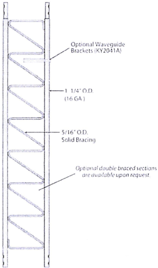
STANDARD SECTION 25G - 10' Section
