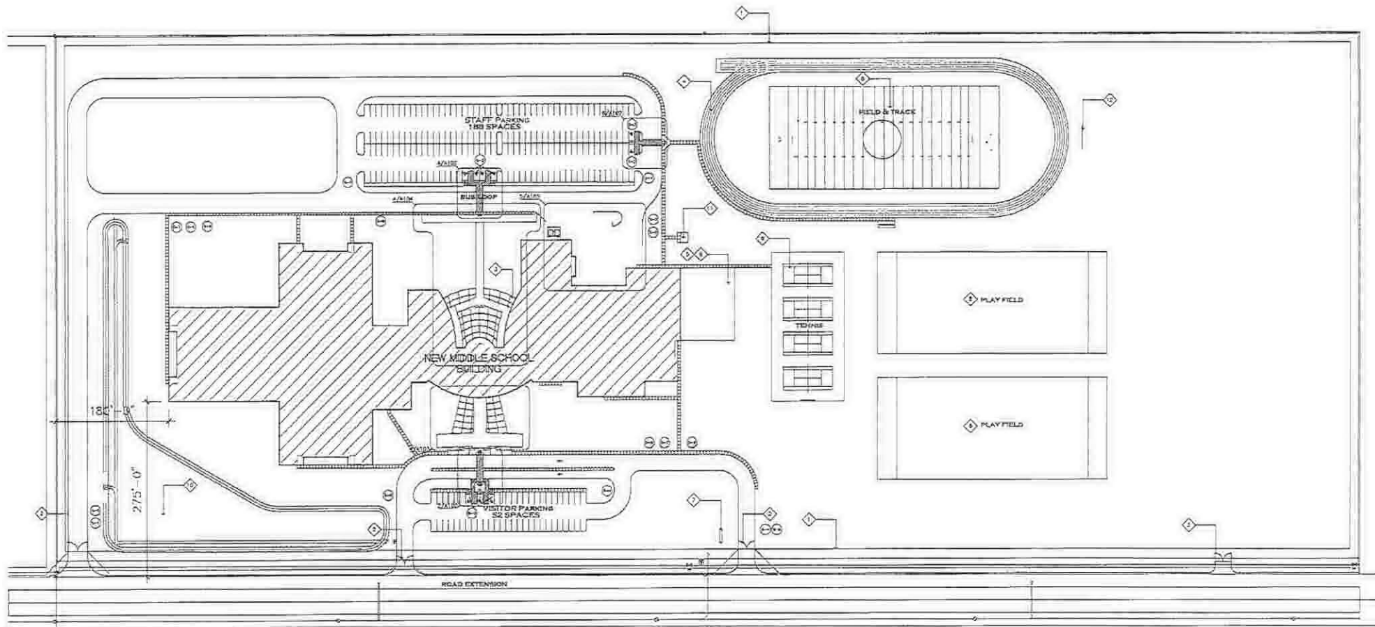
NEW BETTY HARWELL MIDDLE SCHOOL SITE PLAN
