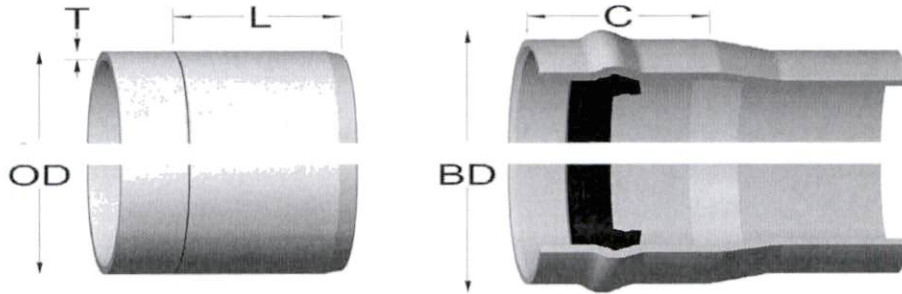
ASTM D3034 GASKETED GRAVITY SEWER PIPE
