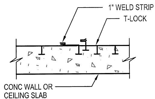
SPLICE
