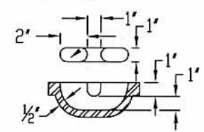
BLIND LIFTING POCKET DETAIL
