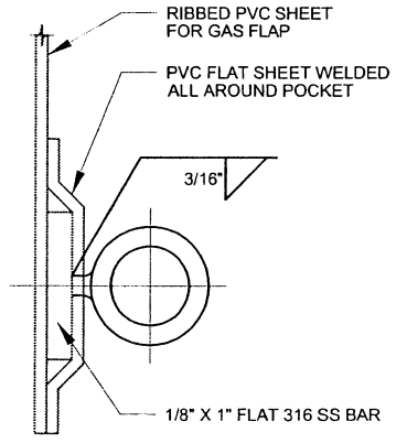
DETAIL 2 NTS
