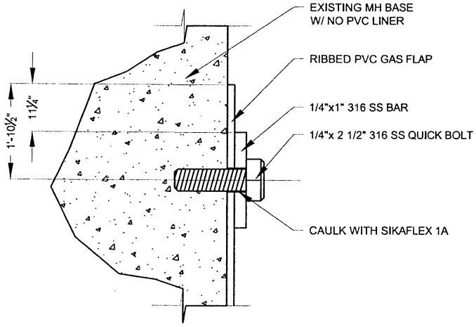
DETAIL 1 NTS
