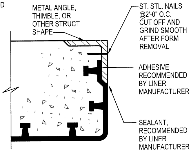
METAL EMBED
