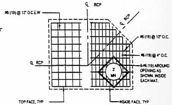
SECTION D NTS TOP SLAB ONLY
