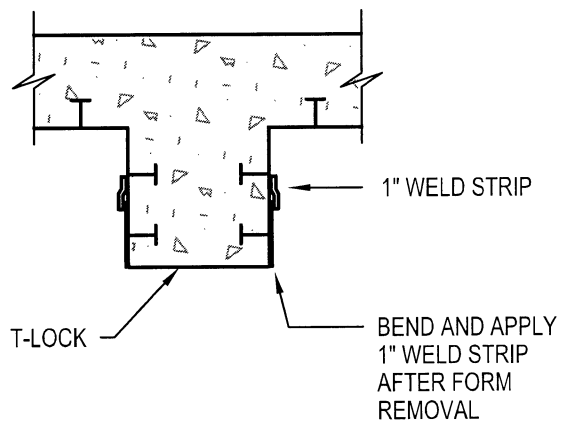
BEAM
