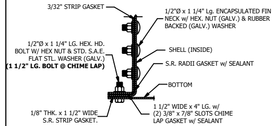
SECTION B-B CHIME BOLTING @ BOTTOM
