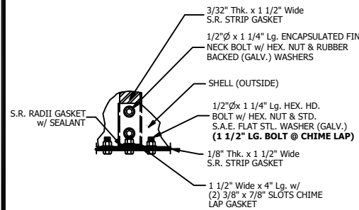
VIEW C S.R. STAVE LAP
