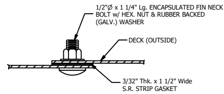
SECTION A-A DECK SEAM LAP
