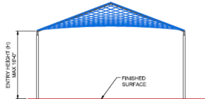
SIDE ELEVATION
