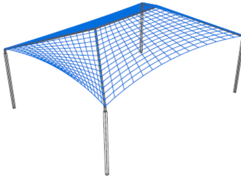
PERSPECTIVE VIEW
