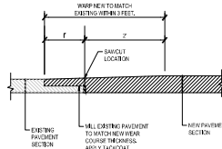
ASPHALT PAVEMENT TRANSITION
