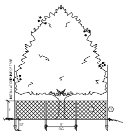
TREE PROTECTION
