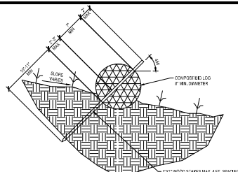
TEMPORARY COMPOST/BIO LOG
