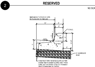
B612 CONCRETE CURB AND GUTTER
