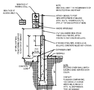
ROUND BOLLARD W/ ACCESSIBLE SIGNAGE MCDONALD'S (MINNESOTA)
