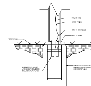
2 BOLLARD BASE DETAIL R6 NO SCALE
