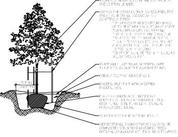
9 DECIDUOUS TREE PLANTING DETAIL
