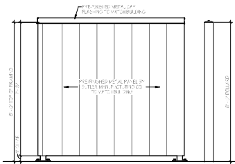
3 TRASH ENCLOSURE ELEVATION 1/2" = 1'-0" 1 / A500
