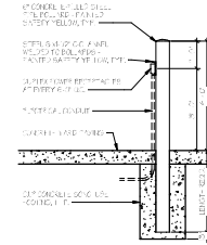
7 CHARGING STATION DETAIL 1/2" = 1'-0" 6 / A500
