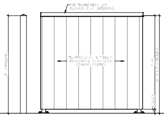
4 TRASH ENCLOSURE ELEVATION 1/2" = 1'-0" 1 / A500
