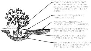
10 SHRUBBERY PLANTING DETAIL
