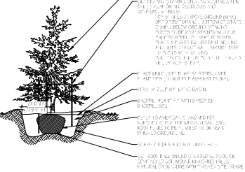
8 CONIFEROUS TREE PLANTING DETAIL
