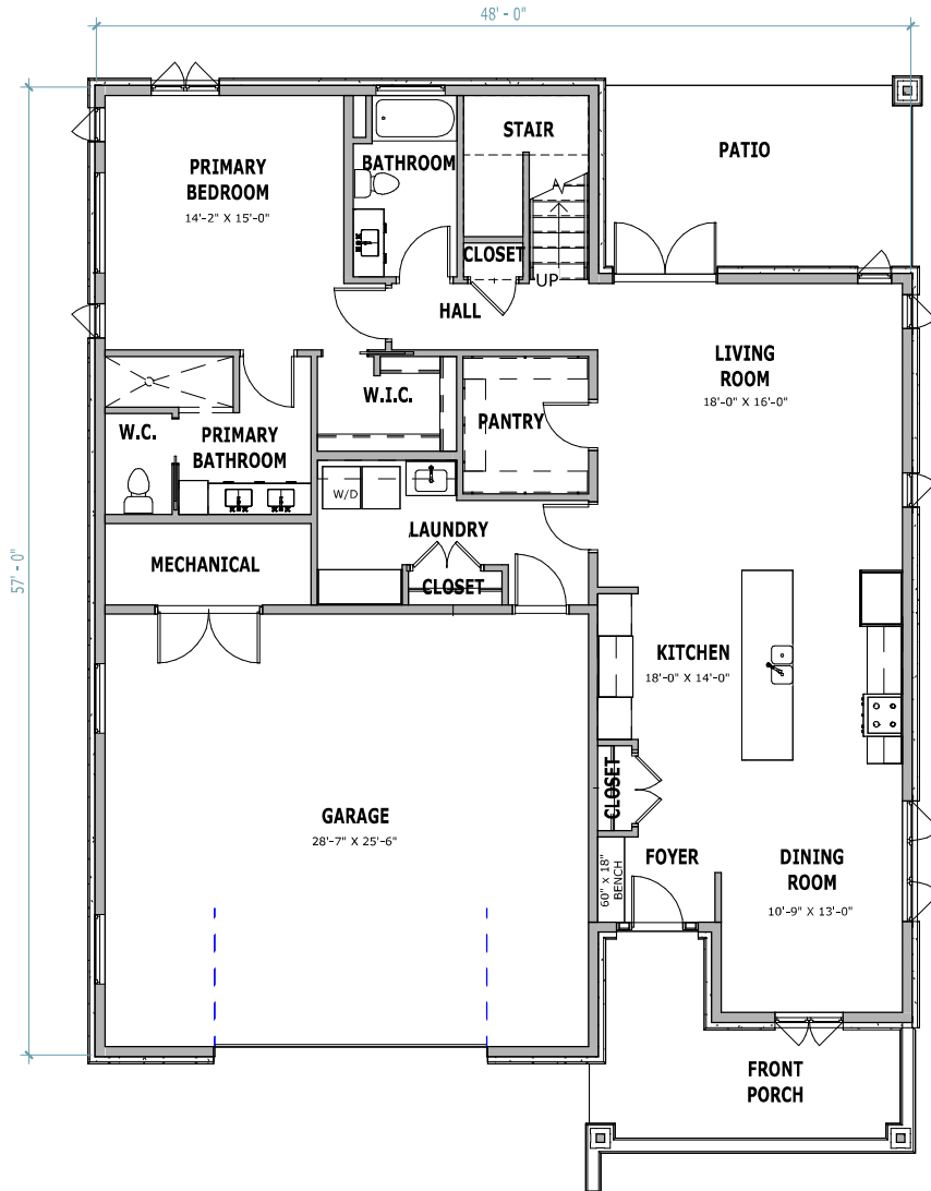
1 MAIN FLOOR 1/8" = 1'-0"
