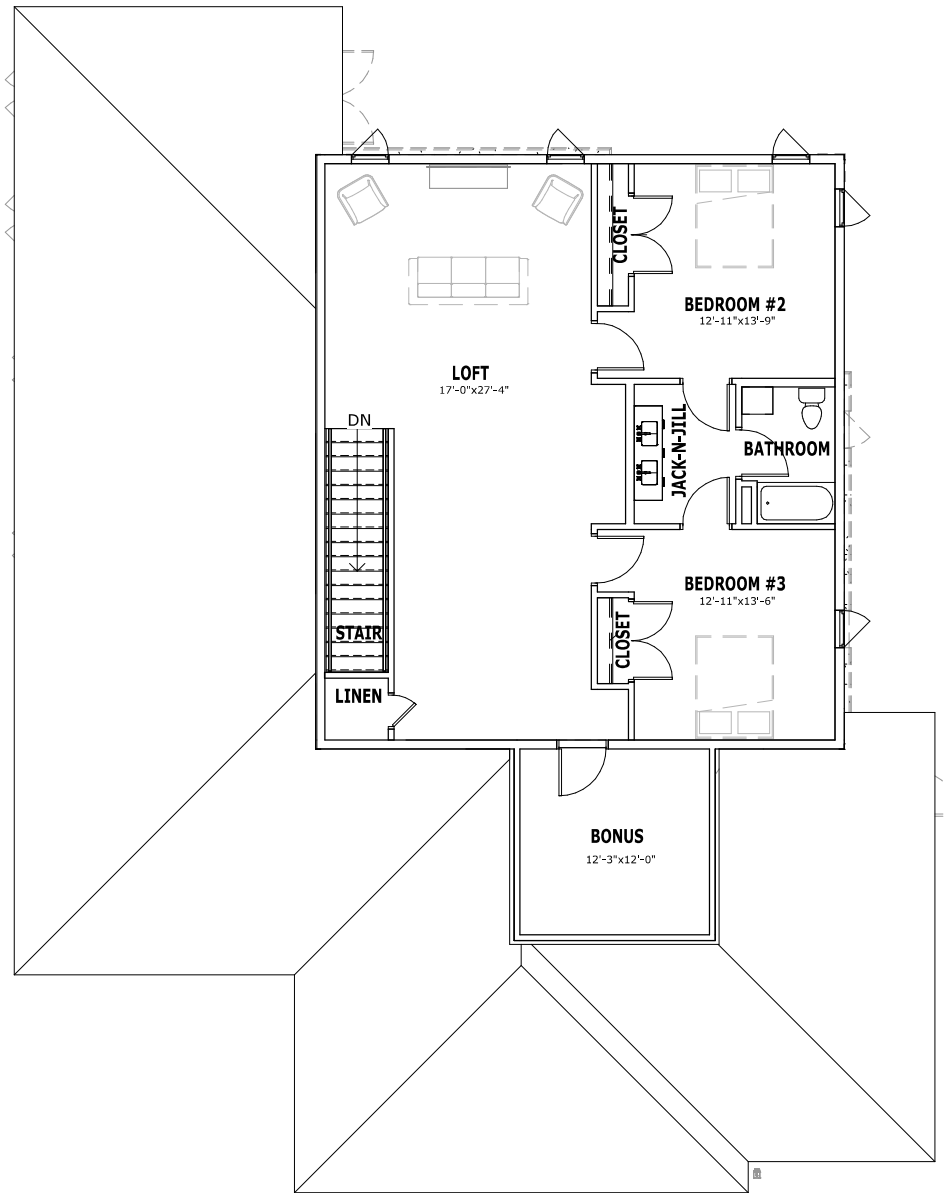
1 SECOND FLOOR - MEDITERRANEAN 1/8" = 1'-0"
