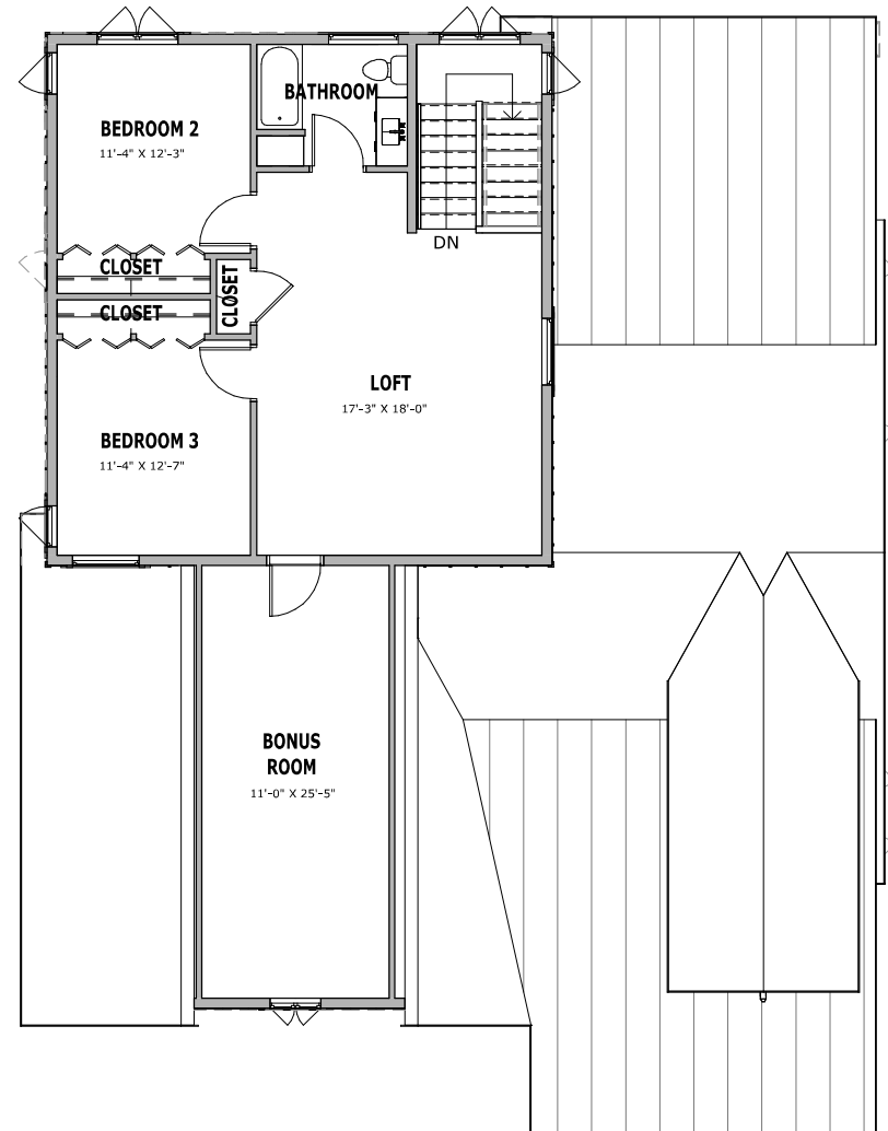
2 SECOND FLOOR 1/8" = 1'-0"
