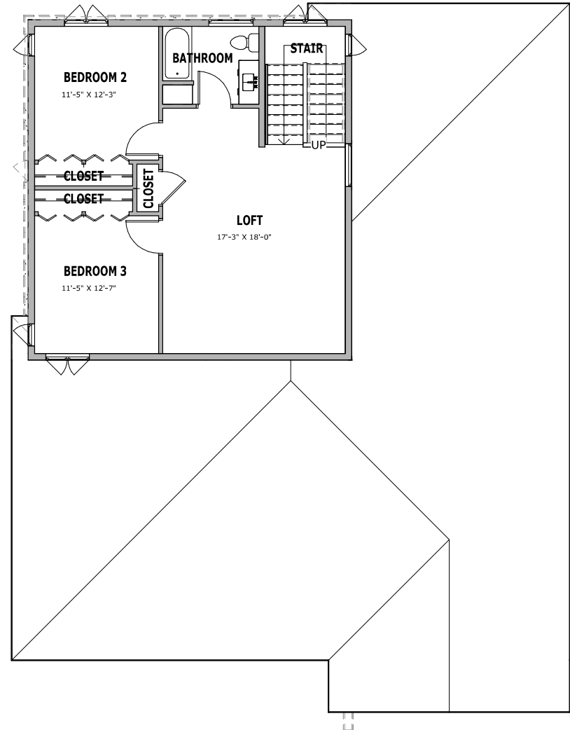
2 SECOND FLOOR 1/8" = 1'-0"
