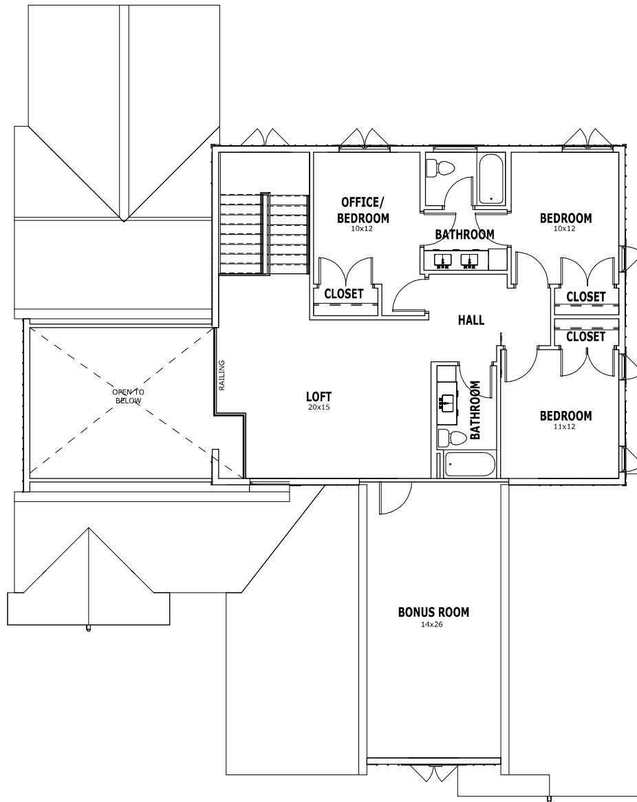
1 SECOND FLOOR PLAN 1/8" = 1'-0"
