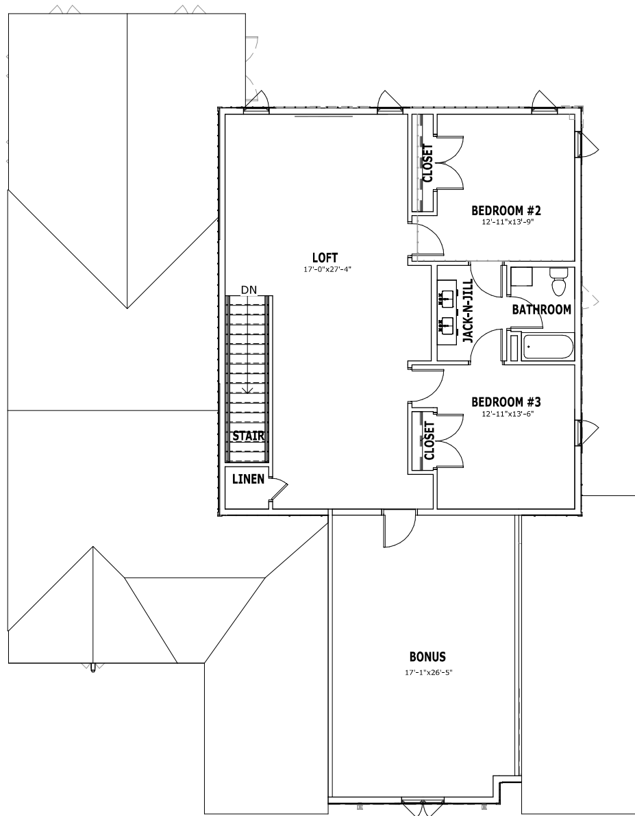
1 SECOND FLOOR - FARMHOUSE 1/8" = 1'-0"
