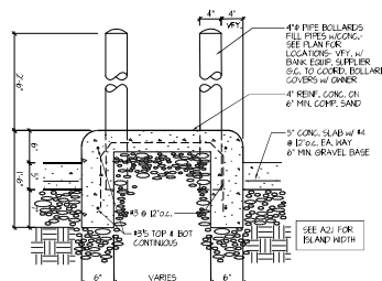
3 TYP. ISLAND DETAIL
