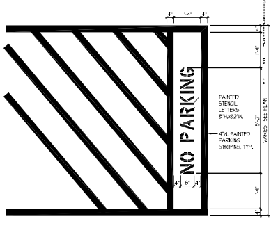
6 TYP. STRIPING DETAIL
