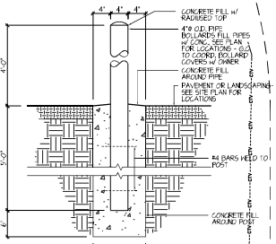
4 TYP. BOLLARD DETAIL
