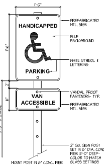
5 HCP SIGN DETAIL
