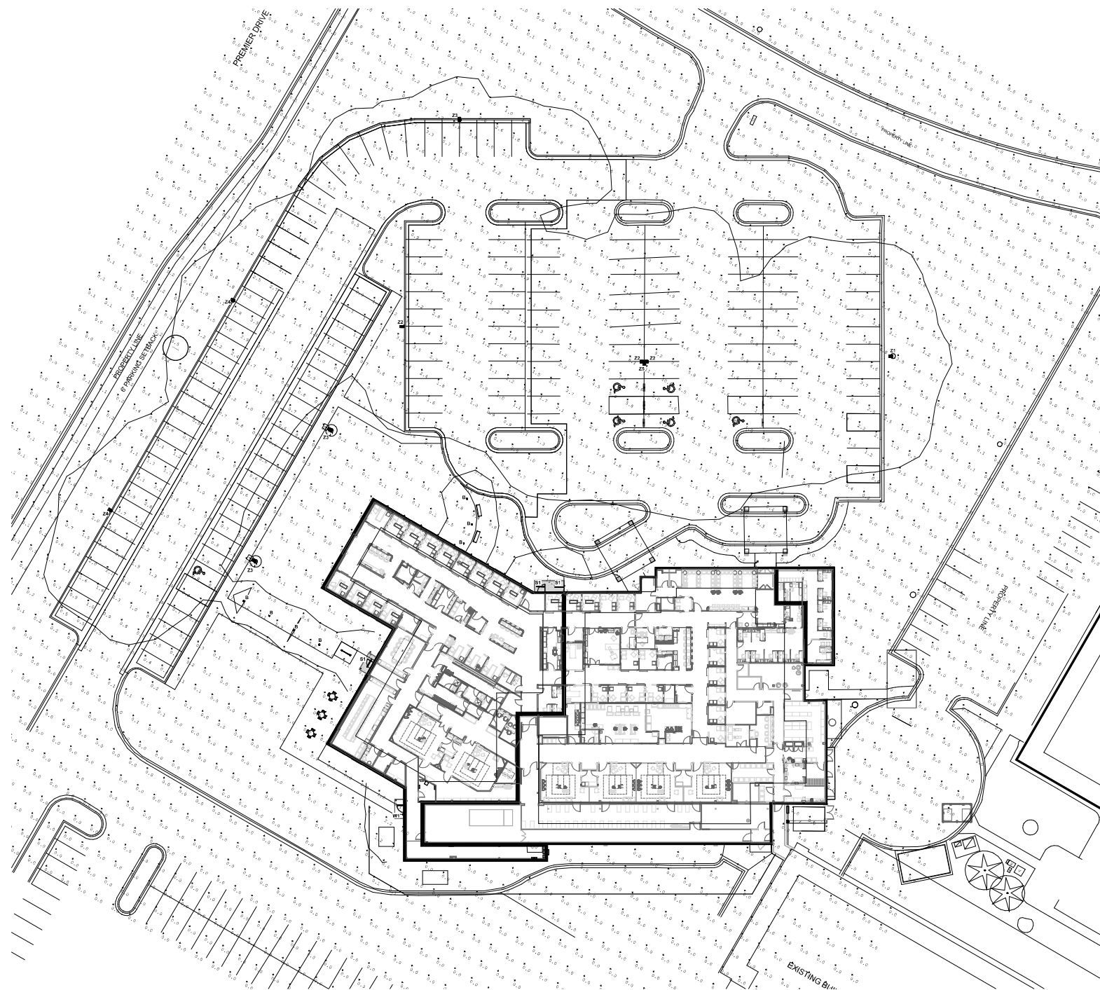
1 SITE PHOTOMETRIC 1/16" = 1'-0"
