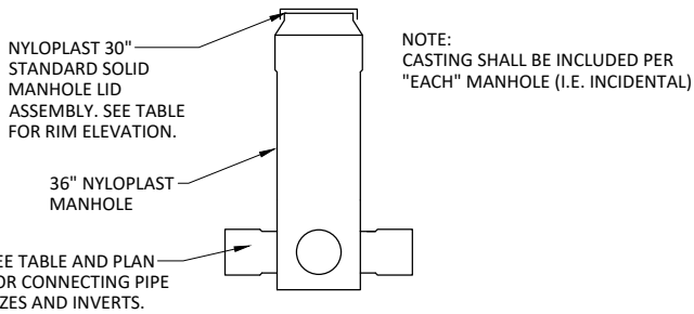
DESIGN SPECIAL - 36" NYLOPLAST MANHOLE NOT TO SCALE
