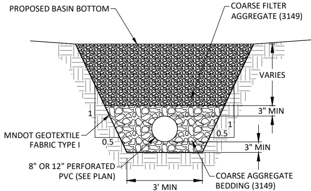
FILTRATION BASIN 8" & 12" PERFORATED PIPE DRAIN NOT TO SCALE
