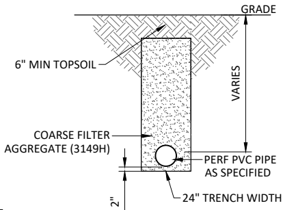
8" PERFORATED PIPE DRAIN NOT TO SCALE
