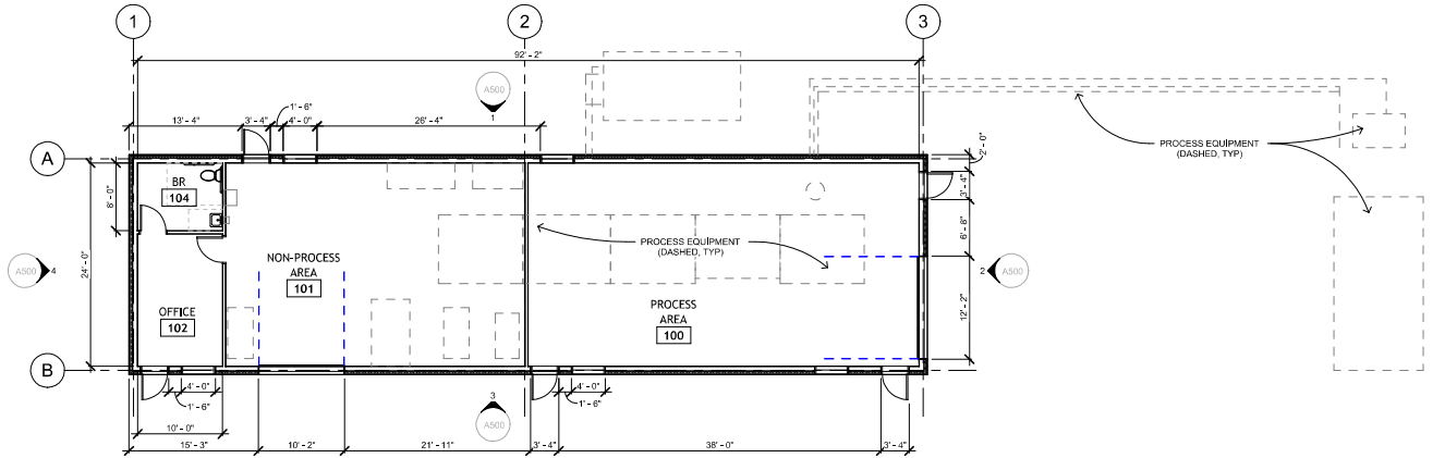
1 LEVEL 1 FLOOR PLAN 1/8" = 1'-0"
