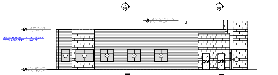
2 SOUTH ELEVATION 1/8" = 1'-0"
