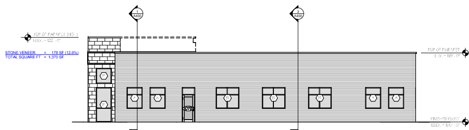
4 NORTH ELEVATION 1/8" = 1'-0"
