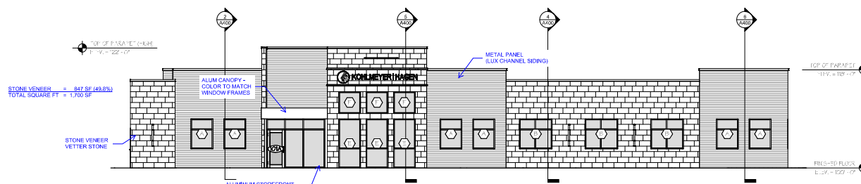
3 EAST ELEVATION 1/8" = 1'-0"
