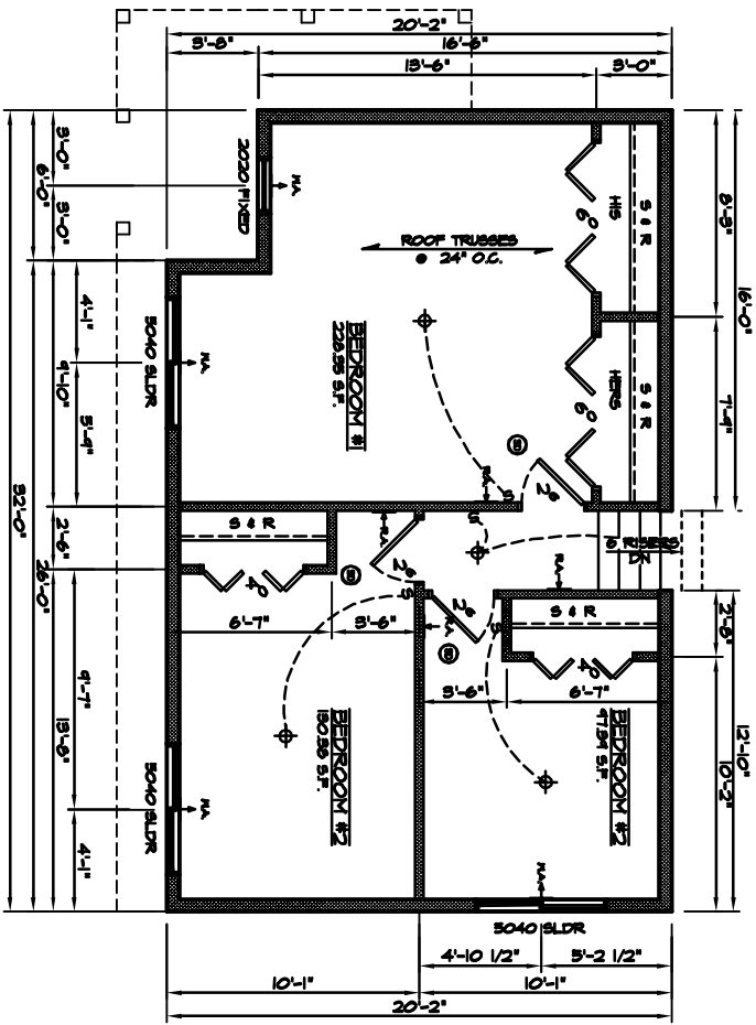
UPPER LEVEL PLAN SCALE: 1/4"=1'-0"
